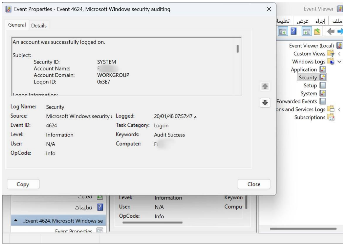
Figure 5. Detailed properties of Event ID 4624
