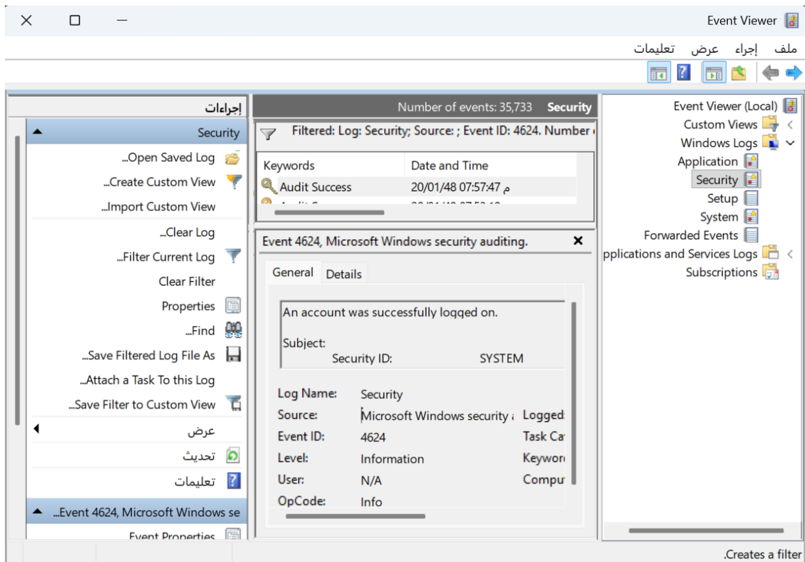
Figure 4. General view of Event ID 4624.
