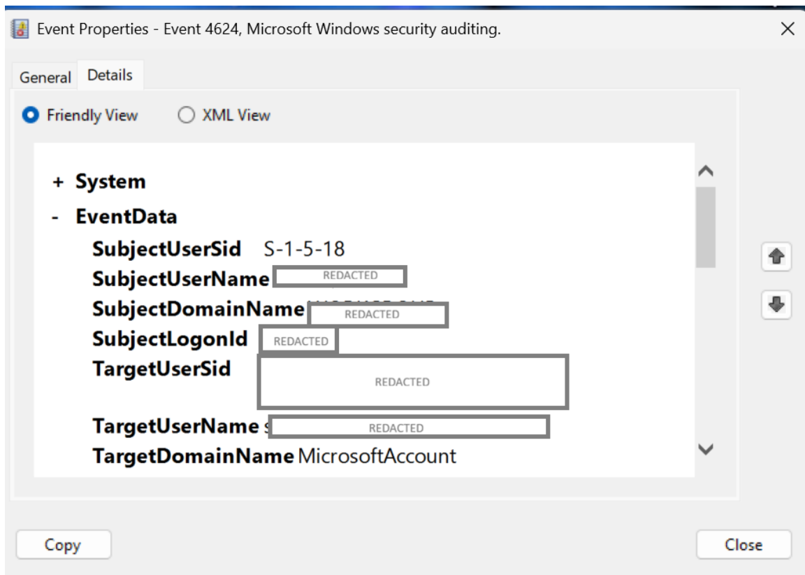
Figure 6. Authentication details for Event ID 4624.
