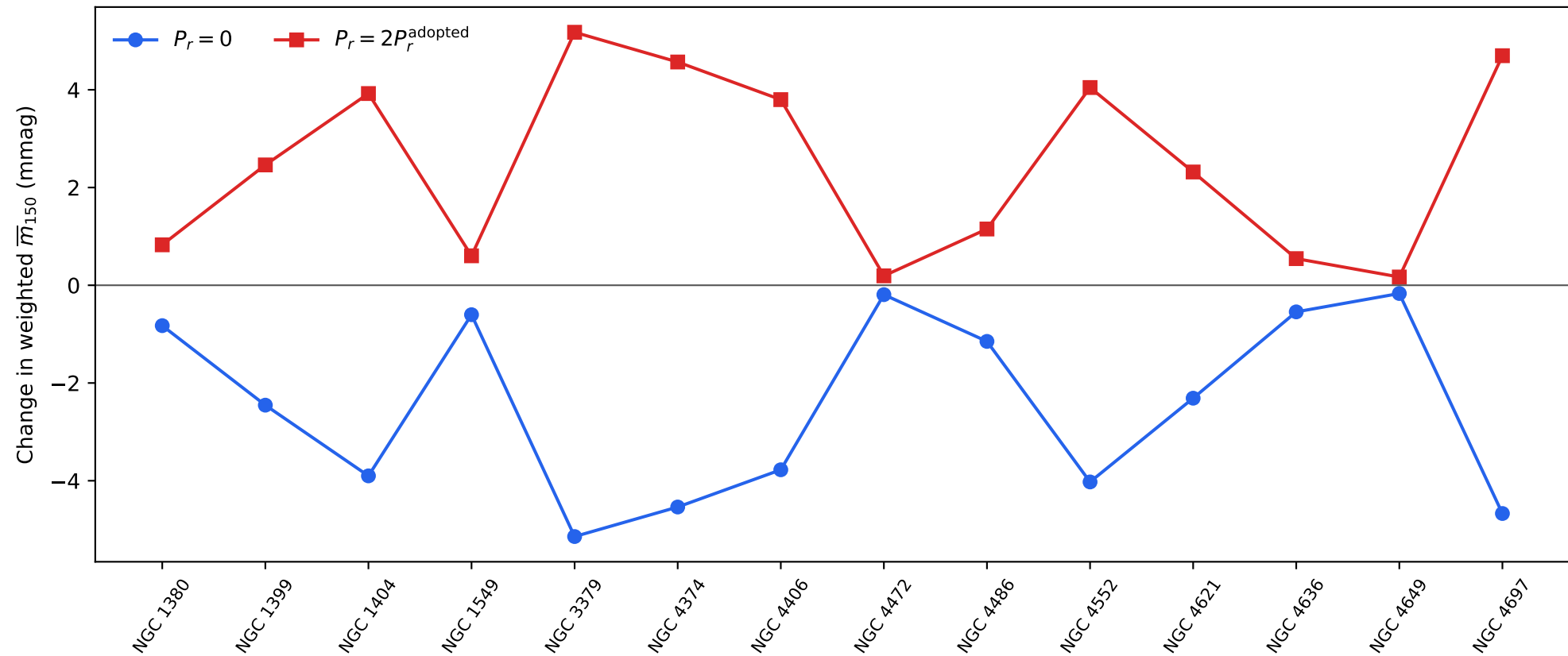
F150W measurement sensitivity to unresolved-source power P_r
