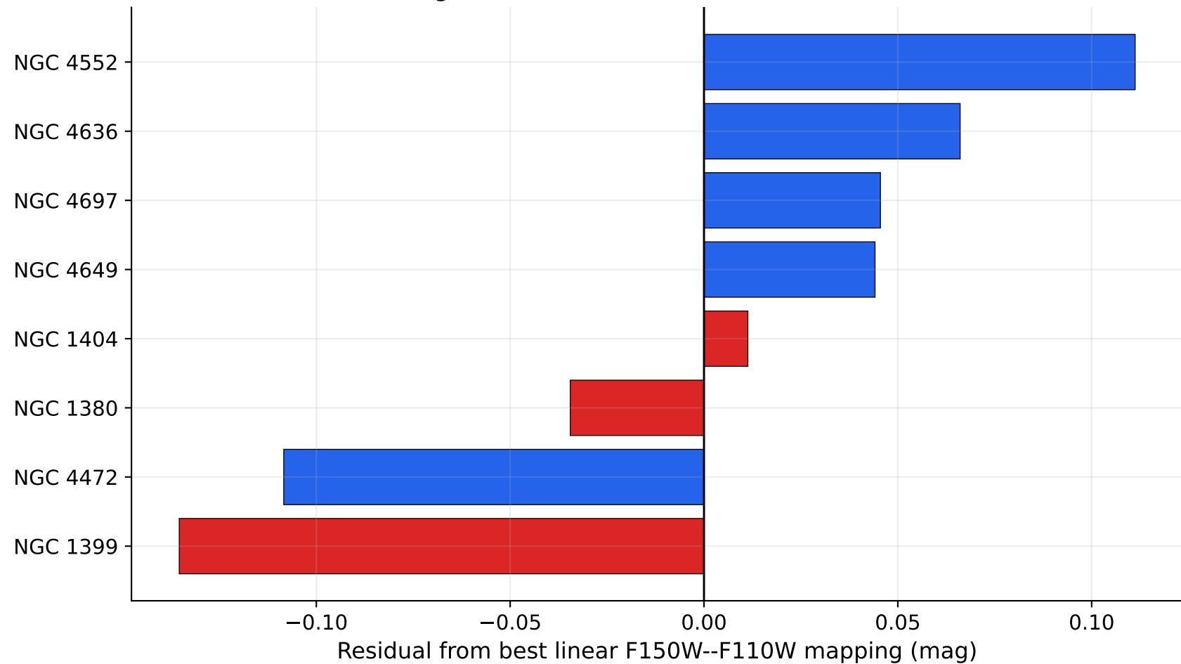
Which galaxies break the cross-filter SBF relation?
