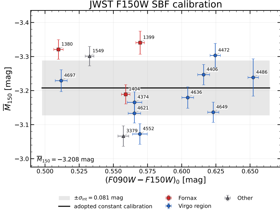
Figure 2: Extinction-corrected JWST F150W SBF calibration. The black horizontal line is the adopted color-independent zero point. The single grey strip is \pm\sigma_{\text{int}} = \pm 0.081 mag around the line; it displays fitted intrinsic scatter, not a confidence interval on the mean or a complete distance error. Red squares denote Fornax, blue circles the broad Virgo-region class, and grey triangles other environments. Numbers identify NGC galaxies. This environment convention is used throughout the galaxy-comparison figures. All 14 objects enter the calibration, irrespective of environment or structural quality. Horizontal bars show the adopted 1\sigma color uncertainty (photometric plus foreground-reddening terms); vertical bars show the individual 1\sigma absolute-SBF calibration-point uncertainty.
