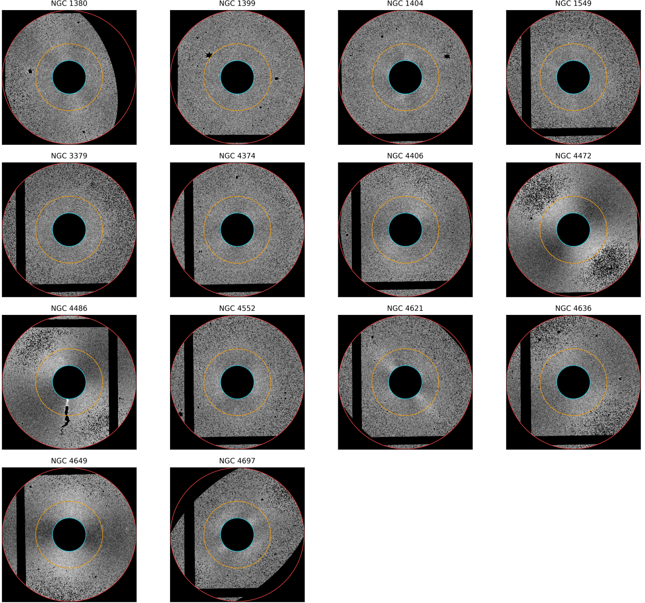
Final normalized F150W FFT inputs: full-support 3.5\sigma winsorization
