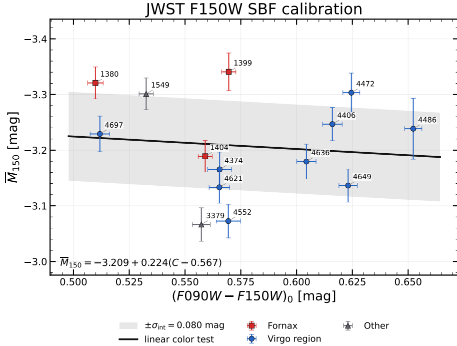
Figure 3: Linear F150W color test for the same 14 galaxies, with the same environment symbols and NGC labels as Figure 2. The line is Eq. 42; the grey strip is \pm\sigma_{\text{int}} = \pm 0.080 mag. The bootstrap slope interval includes zero, and the linear model worsens LOO RMS from 0.0925 to 0.0981 mag. Thus the color term is not required by these data; this is a model-comparison result, not a claim that the linear function is mathematically invalid. Horizontal and vertical bars have the same 1\sigma definitions as in Figure 2.
