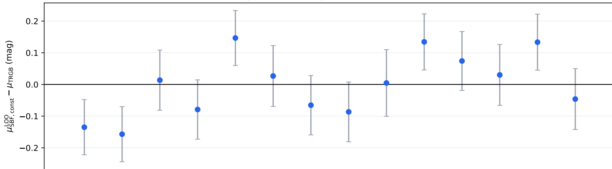
Adopted color-independent LOO residuals
