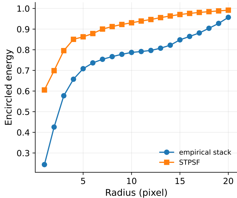
Diagnostic delta m = +0.288 mag
