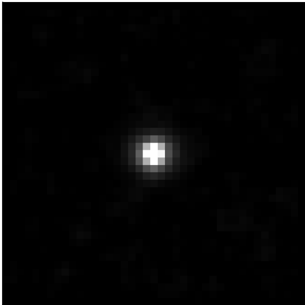
NGC 3379 empirical stack (n=6)
