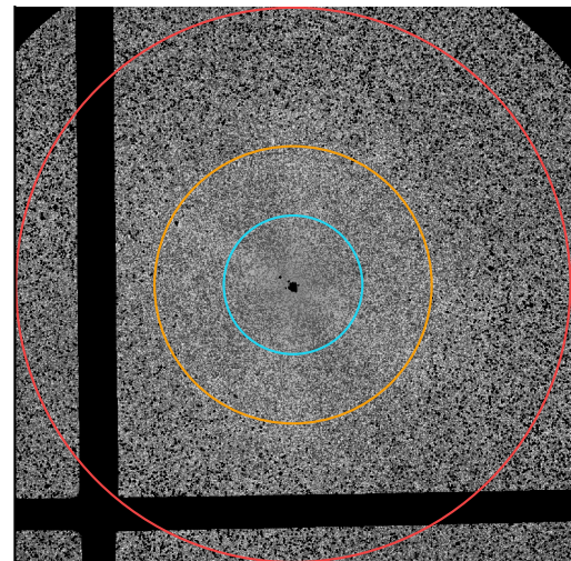
NGC 4472
