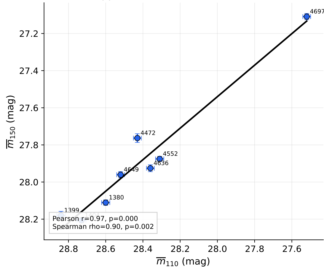
Apparent SBF: distance dominated
