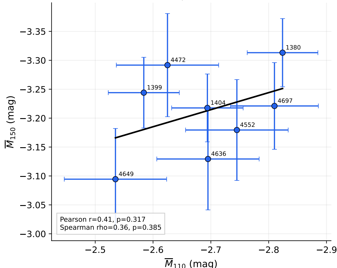
Absolute SBF: Paper III cluster anchor
