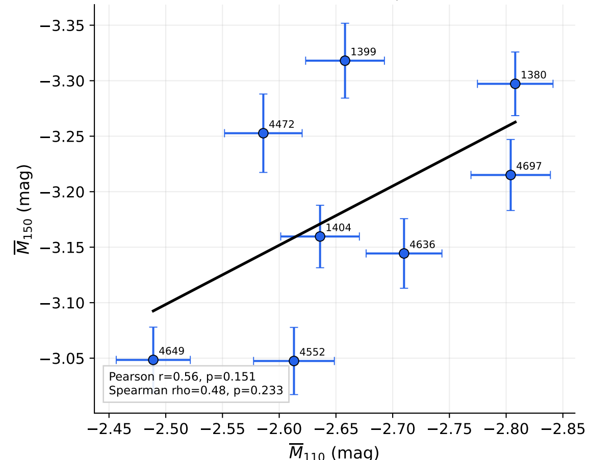
Absolute SBF: individual Paper IV anchor
