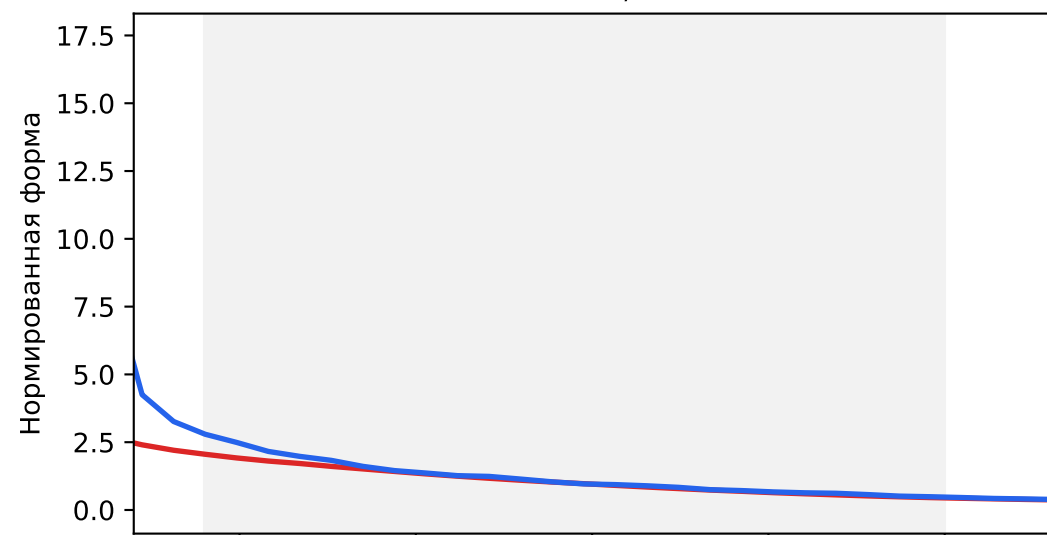
NGC 4486, inner
