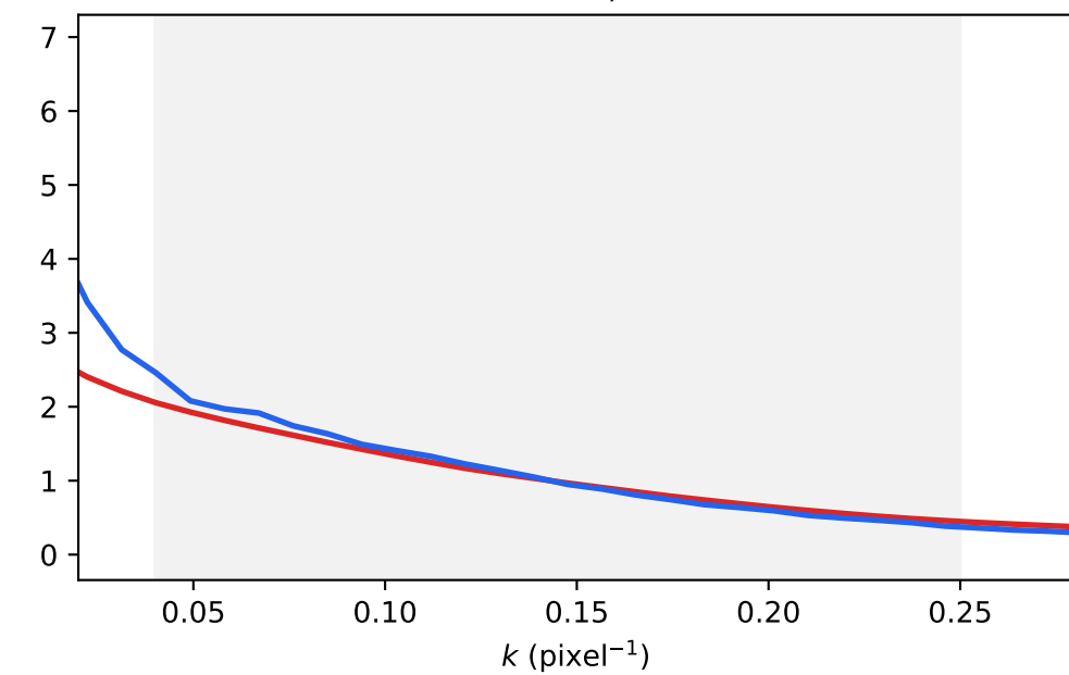
NGC 4486, outer
