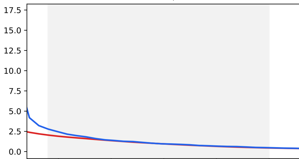
NGC 4486, outer
