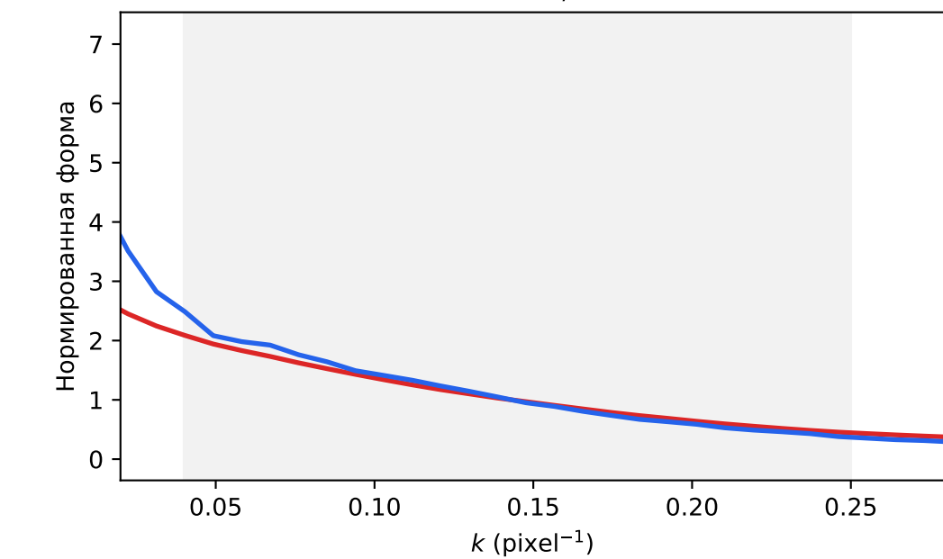
NGC 4486, inner
