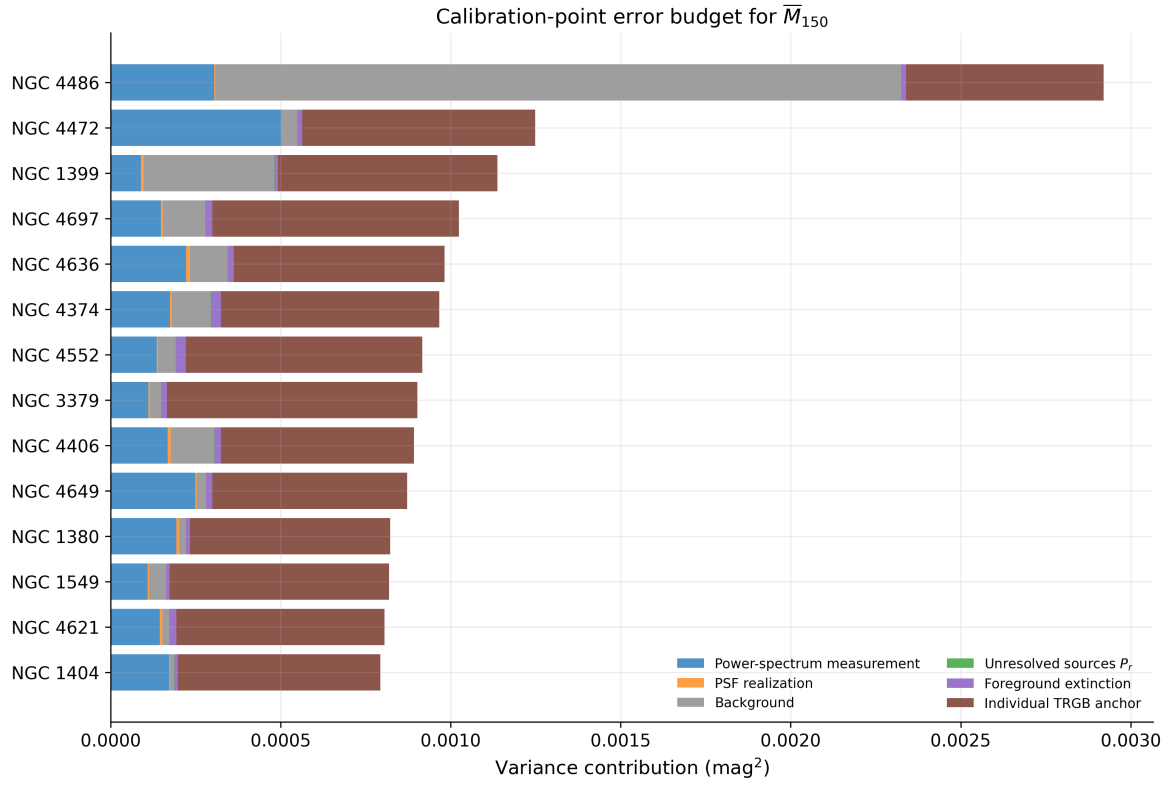
Figure 5: Variance budget of each absolute F150W calibration point. Stacked segments are the contributions to \sigma_{\overline{M}}^2 from the power-spectrum fit, sky, PSF realization, unresolved-source correction, foreground extinction, and individual TRGB anchor. The horizontal scale is variance in \text{mag}^2 , not a magnitude error; the total 1\sigma uncertainty is the square root of the complete bar.
