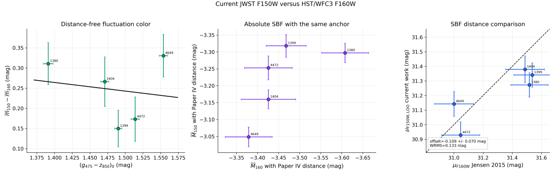
Figure 13: Comparison with the five independently reduced Jensen et al. (2015) F160W overlaps. The sample is too small for a new calibration claim; the plot is retained only as the separately labelled cross-band consistency check described in the main text. The black line in the left panel is the fitted fluctuation-color trend; the dashed black line in the right panel is equality. The middle panel has no fitted black line.
