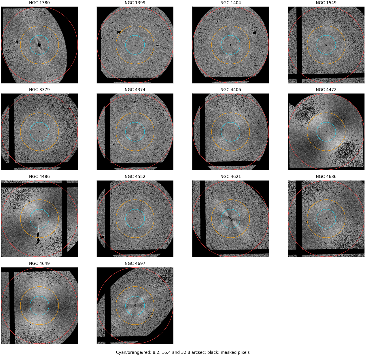
Figure 1: Final normalized F150W residual fields used for the SBF measurement. The smooth galaxy model has been subtracted, compact sources and invalid image regions have been masked, and the two adopted circular annuli are retained. Black pixels are excluded from the analysis; visible grey-scale structure in the unmasked area is real residual structure, not a mask value.
