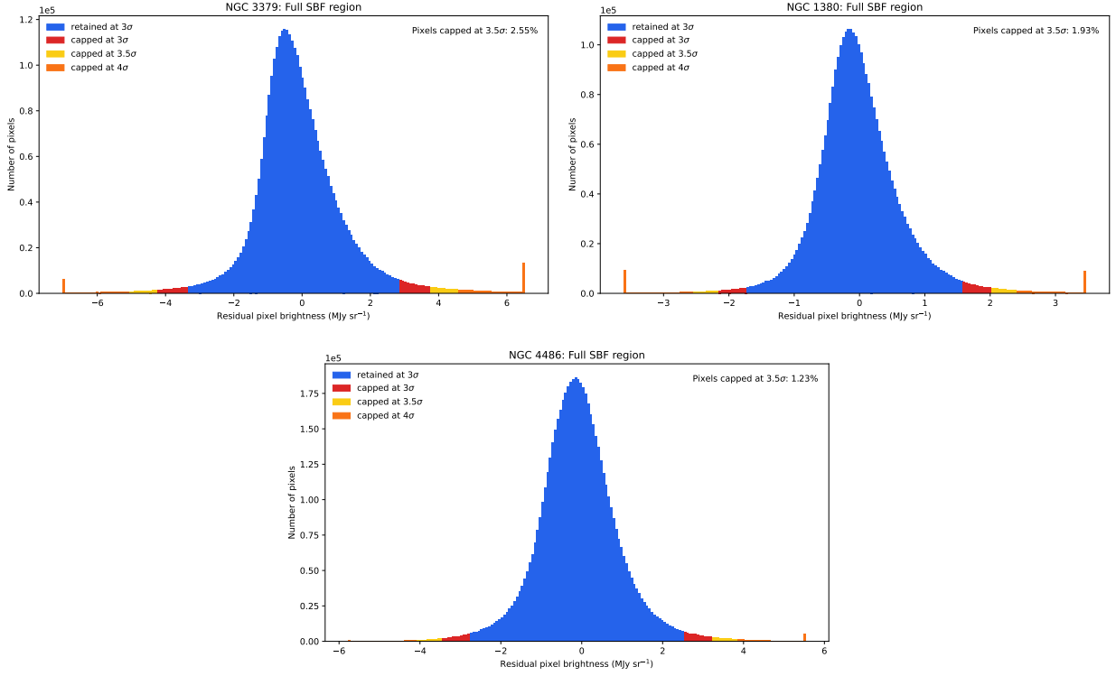
Figure 10: Full-SBF-region residual-pixel distributions for the three representative winsorization tests. The colored tails mark values modified by the 3, 3.5, and 4\sigma limits; the adopted 3.5\sigma boundary changes only 1.23–2.55 per cent of all region pixels, although the exact P(k) refits show that the inner annulus remains sensitive to these rare tails.
