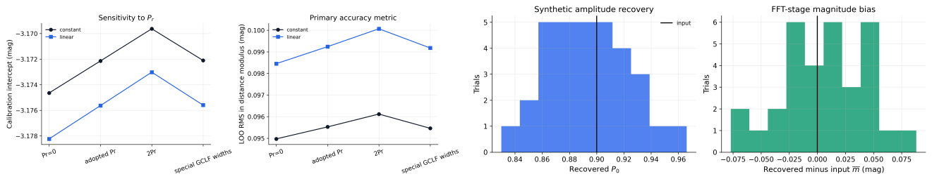
Figure 12: Left: calibration and color-independent LOO metric under the P_r sensitivity experiments. Right: recovery of known P_0 and SBF magnitude in the synthetic FFT-stage test.
