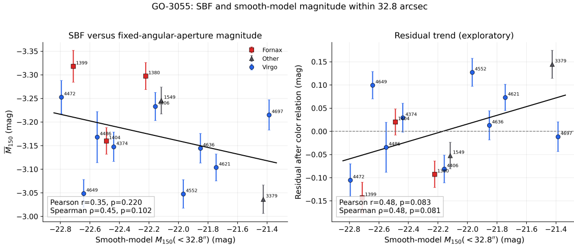
Figure 14: F150W SBF versus the smooth-model magnitude inside the fixed 32.8-arcsec aperture. This quantity is an aperture luminosity, not a total galaxy magnitude, and the same angular radius covers different physical radii. The right panel subtracts the rejected linear color relation only as an exploratory diagnostic; neither panel enters the adopted distance estimator.
