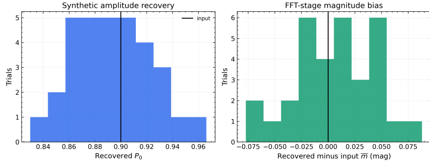
Figure 21: Recovery of known P_0 and SBF magnitude in the synthetic FFT-stage test. A representative F150W PSF is used to test the common Fourier normalization and unit conversion; this is not a separate estimate of an F150W-only systematic.
