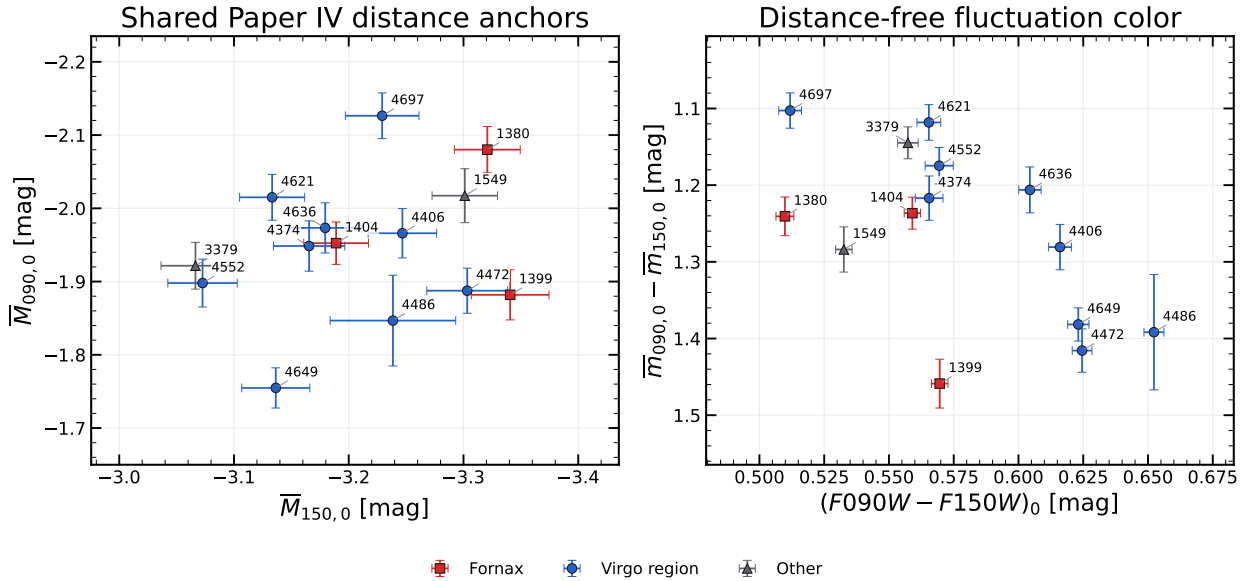
Figure 24: Direct comparison of the independently measured F090W and F150W fluctuation quantities for the same 14 galaxies. The panels are cross-band diagnostics and do not constitute an independent distance validation because both analyses use the same galaxies, angular regions, two-band color photometry, and TRGB anchors. The signal images, fitted galaxy models, and source masks themselves are band specific.
