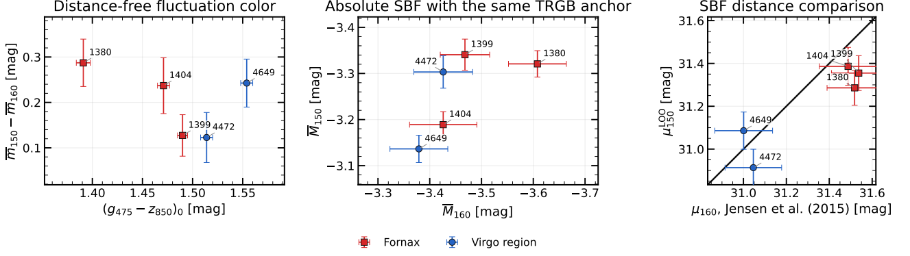
Figure 22: Comparison with the five independently reduced Jensen et al. (2015) F160W overlaps for the F150W measurements. From left to right: the distance-free fluctuation color, absolute SBF magnitudes using the same TRGB anchor, and LOO SBF distance moduli. The black line in the right panel is equality. The five-object sample is retained as a cross-band consistency check and does not define a new calibration.
