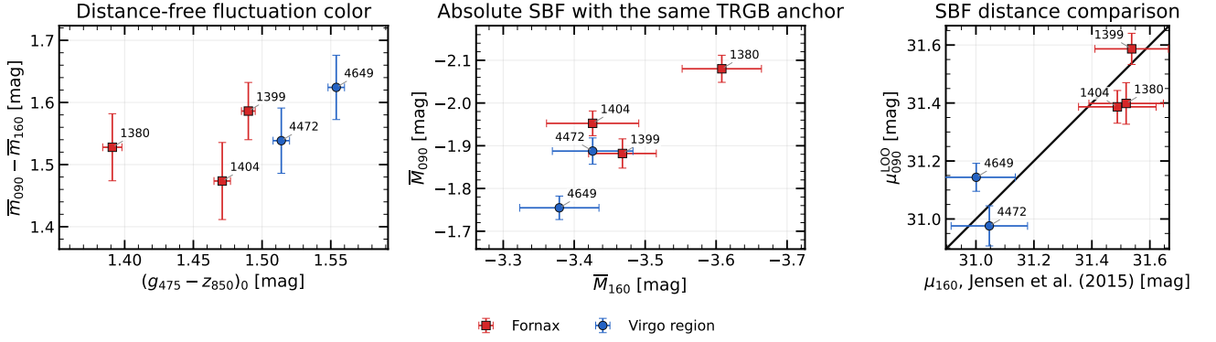
Figure 23: The direct F090W counterpart of Figure 22, using the same five Jensen et al. (2015) F160W overlaps and the same three comparisons. This diagnostic likewise does not enter the adopted F090W calibration.
