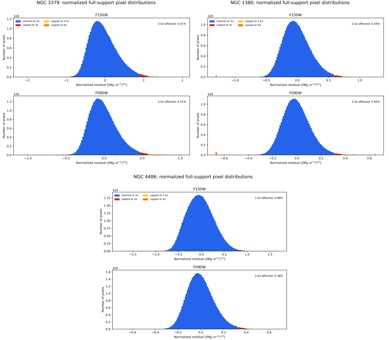
Figure 18: Normalized full-support pixel distributions before winsorization, reconstructed from the final model and mask products for three representative galaxies. Each target is shown in F150W and F090W. Blue is the central region retained by a 3\sigma rule; red, yellow, and orange mark the successive 3\sigma , 3.5\sigma , and 4\sigma tails. The adopted 3.5\sigma threshold affects less than one per cent of valid pixels in these examples. Values beyond the displayed range are accumulated in the edge bins, not discarded from the pixel count. a
