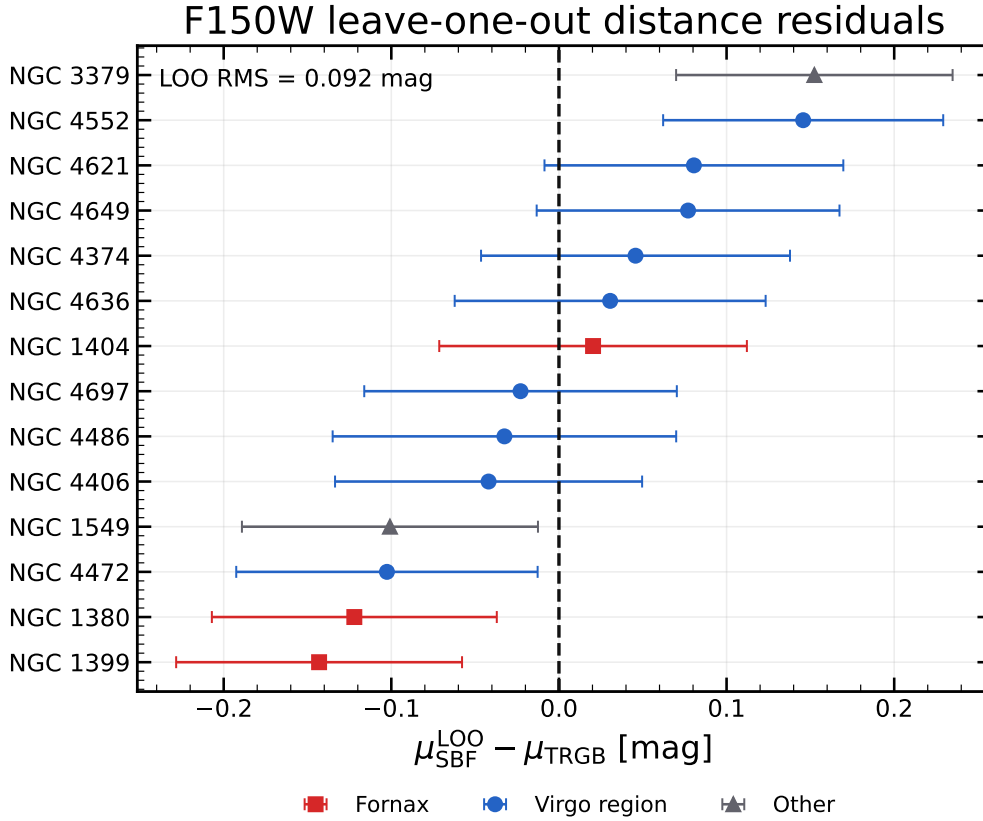
Figure 6: Residuals of the color-independent F150W LOO predictions relative to the individual Paper IV thin-slice TRGB moduli. The vertical dashed line marks zero residual. Error bars contain the galaxy-dependent predictive terms but exclude the shared absolute TRGB zero-point scale.
