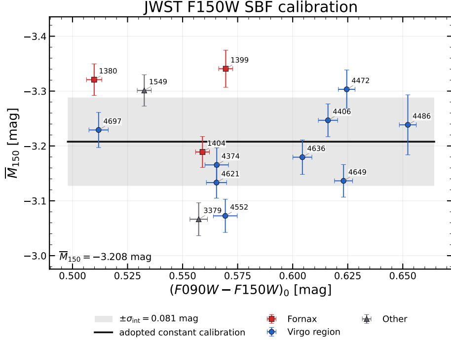
Figure 2: Extinction-corrected JWST F150W SBF calibration. The black horizontal line is the adopted color-independent zero point. The single grey strip is \pm\sigma_{\text{int}} = \pm 0.081 \text{ mag} around the line; it displays fitted intrinsic scatter, not a confidence interval on the mean or a complete distance error. Red squares denote Fornax, blue circles the broad Virgo-region class, and grey triangles other environments. Numbers identify NGC galaxies. This environment convention is used throughout the galaxy-comparison figures. All 14 objects enter the calibration, irrespective of environment or structural quality. Horizontal bars show the adopted 1\sigma color uncertainty (photometric plus foreground-reddening terms); vertical bars show the individual 1\sigma absolute-SBF calibration-point uncertainty.
