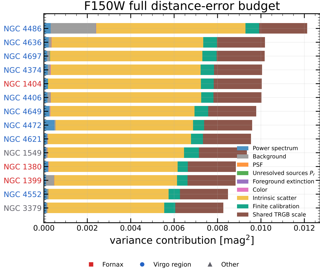
Figure 8: Full F150W LOO distance-error budget in the same variance representation. In addition to the image-measurement terms, the bars include intrinsic calibration scatter, finite-sample calibration uncertainty, and the shared TRGB absolute scale. The latter is coherent between galaxies and must not be interpreted as 14 independent random contributions.
