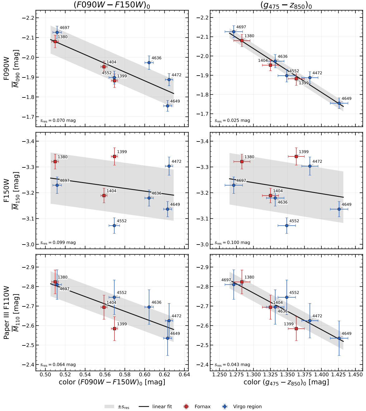
Figure 4: Same-galaxy color test for the eight objects common to this work and Paper III. Rows show F090W, F150W, and Paper III F110W; columns use F090W - F150W and g - z . Thus neither the galaxy list nor the color tracer is changed in isolation. F090W and F110W retain clear slopes, whereas F150W does not. Each single grey strip shows \pm s_{\text{res}} around its ordinary least-squares line, where s_{\text{res}}^2 = \sum_i (y_i - \hat{y}_i)^2 / (8 - 2) . This is observed residual scatter, including measurement noise, rather than the fitted intrinsic scatter or a confidence interval for the coefficients. Red squares denote Fornax and blue circles the broad Virgo-region class; every point is labelled by its NGC number.
