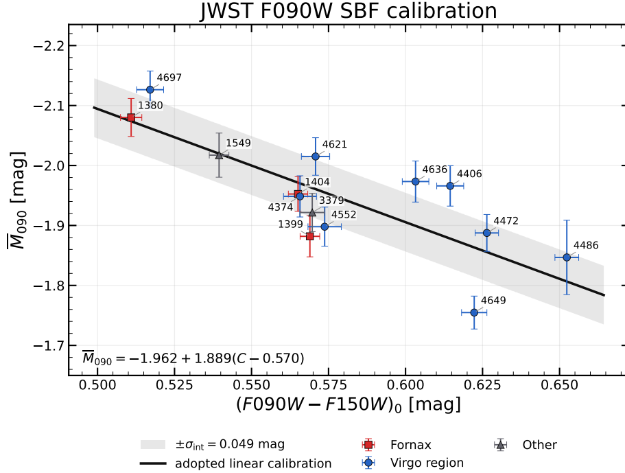
Figure 10: Adopted F090W color calibration. Points are the 14 individual \overline{M}_{090} calibration measurements and the black line is Eq. 43. The single grey strip is \pm\sigma_{\text{int}} = \pm 0.049 mag around the line. It visualizes intrinsic scatter, not coefficient uncertainty or the full predictive distance error. Environment colors, symbols, and NGC labels follow Figure 2; all 14 objects enter the fit. Horizontal bars show the adopted 1\sigma color uncertainty; vertical bars show the individual 1\sigma absolute-SBF calibration-point uncertainty.
