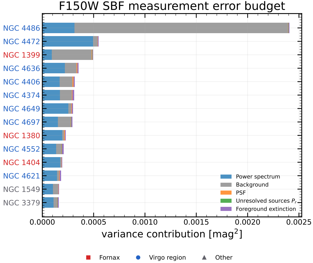
Figure 7: F150W apparent-SBF measurement budget in a stacked variance representation. Each horizontal segment is one contribution \sigma_i^2 ; the total measurement uncertainty is the square root of the complete bar length. Galaxies are ordered by total measurement variance.
