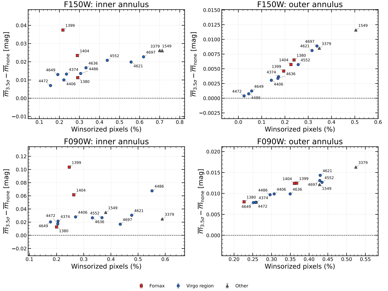
Figure 17: Matched all-galaxy test of the adopted normalized-space 3.5\sigma winsorization. The upper row is F150W and the lower row is F090W. Left panels show the inner annulus and right panels the outer annulus. The ordinate is the SBF-magnitude change relative to no winsorization; the abscissa is the percentage of affected pixels. Environment symbols follow Figure 2, with every galaxy identified by its NGC number. These percentages describe changed pixels, not a confidence level. All values come from the final full-support products.
