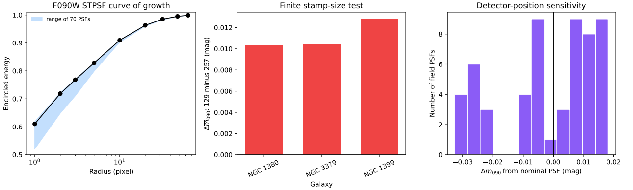
Figure 16: Direct F090W counterpart of Figure 15, with the same encircled-energy, 129-versus-257-pixel, and detector-position tests. The panels use the same final annular weighting and fitted frequency range.
