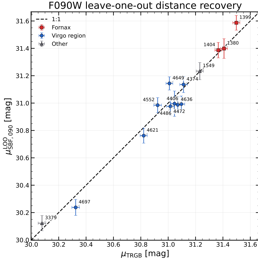
Figure 11: Color-dependent F090W LOO distance moduli compared with the individual Paper IV thin-slice TRGB moduli. Each target is excluded from its own calibration and the dashed line is equality. Error bars are internal; the common absolute zero point is not shown.
