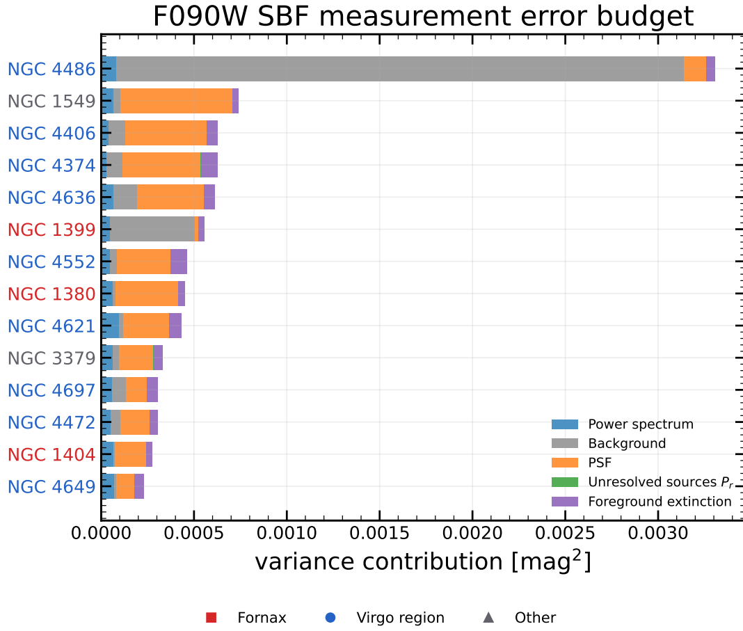
Figure 13: F090W apparent-SBF measurement budget in the same variance representation as Figure 7. Each horizontal segment is one contribution \sigma_i^2 and galaxies are ordered by total measurement variance.
