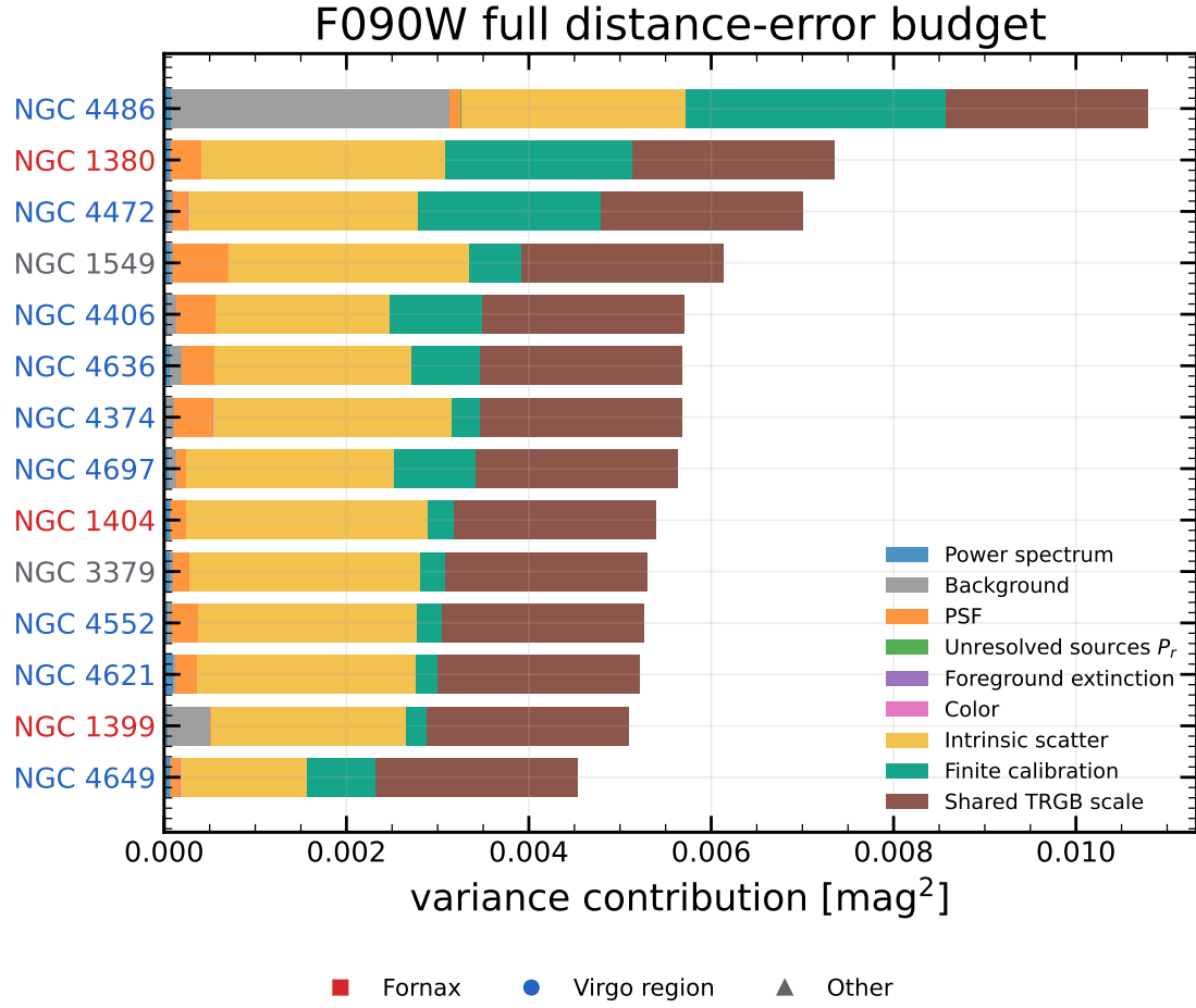
Figure 14: Full F090W LOO distance-error budget in the same variance representation as Figure 8. The color-propagation term is included for the adopted linear calibration; intrinsic scatter, finite calibration, and the coherent TRGB absolute scale are added as distinct components.
