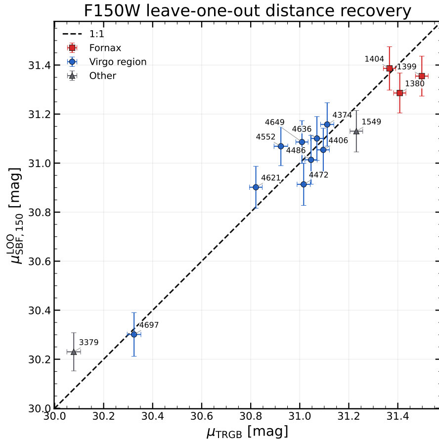
Figure 5: Color-independent LOO F150W SBF distance moduli compared with the individual Paper IV thin-slice TRGB moduli. Each target is excluded from its own calibration. The dashed line is equality. Error bars are internal; the common absolute zero point is not shown.
