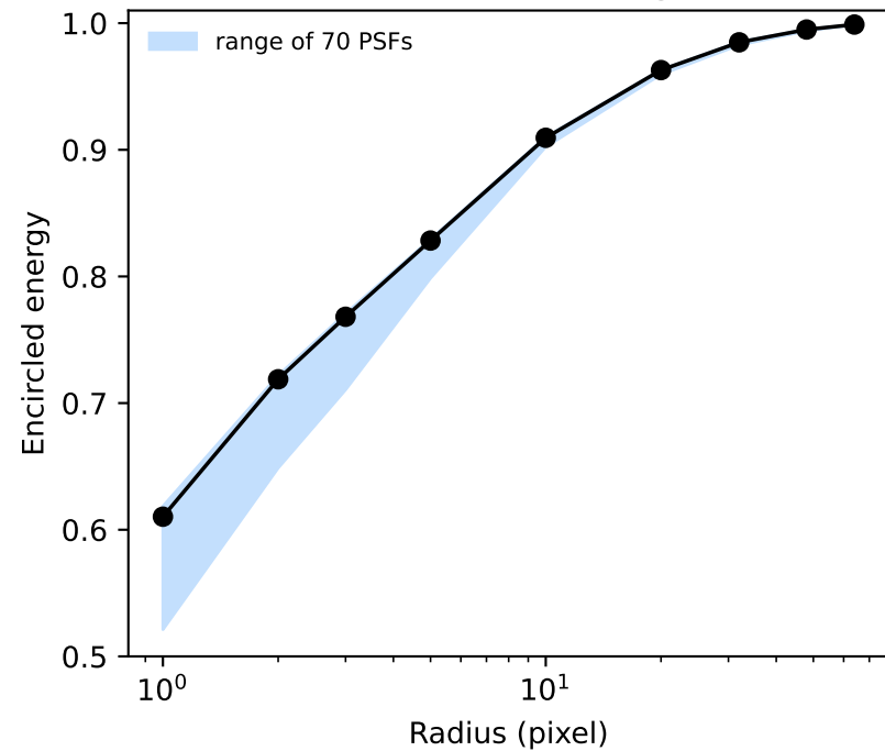
F090W STPSF curve of growth
