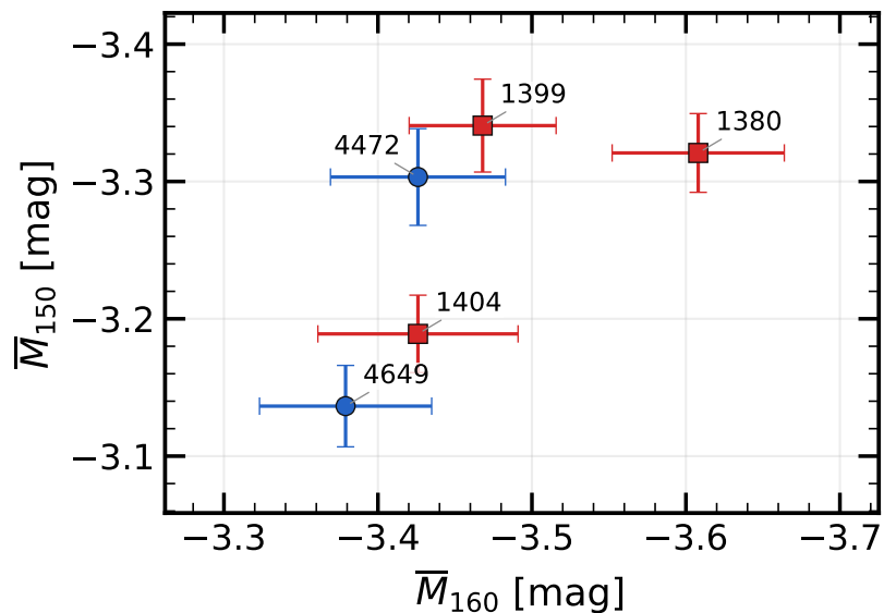
Absolute SBF with the same TRGB anchor
