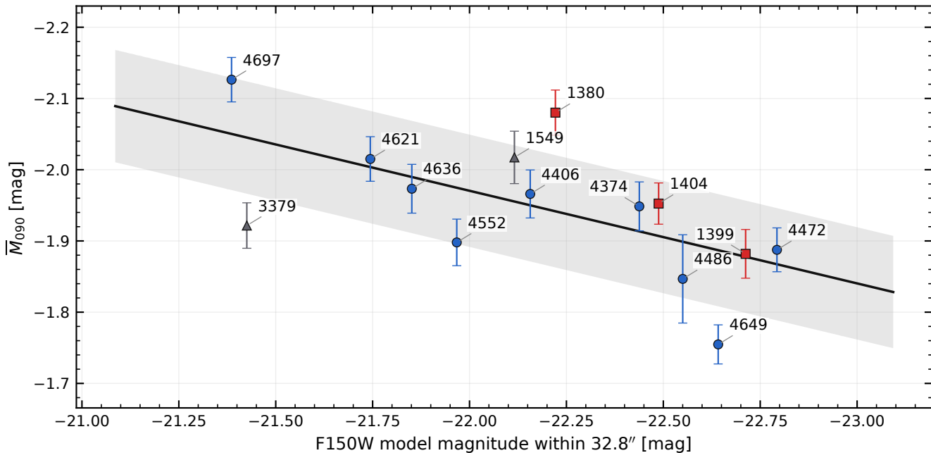
F090W SBF versus host aperture magnitude
