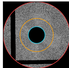
NGC 4472
