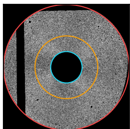
NGC 4649
