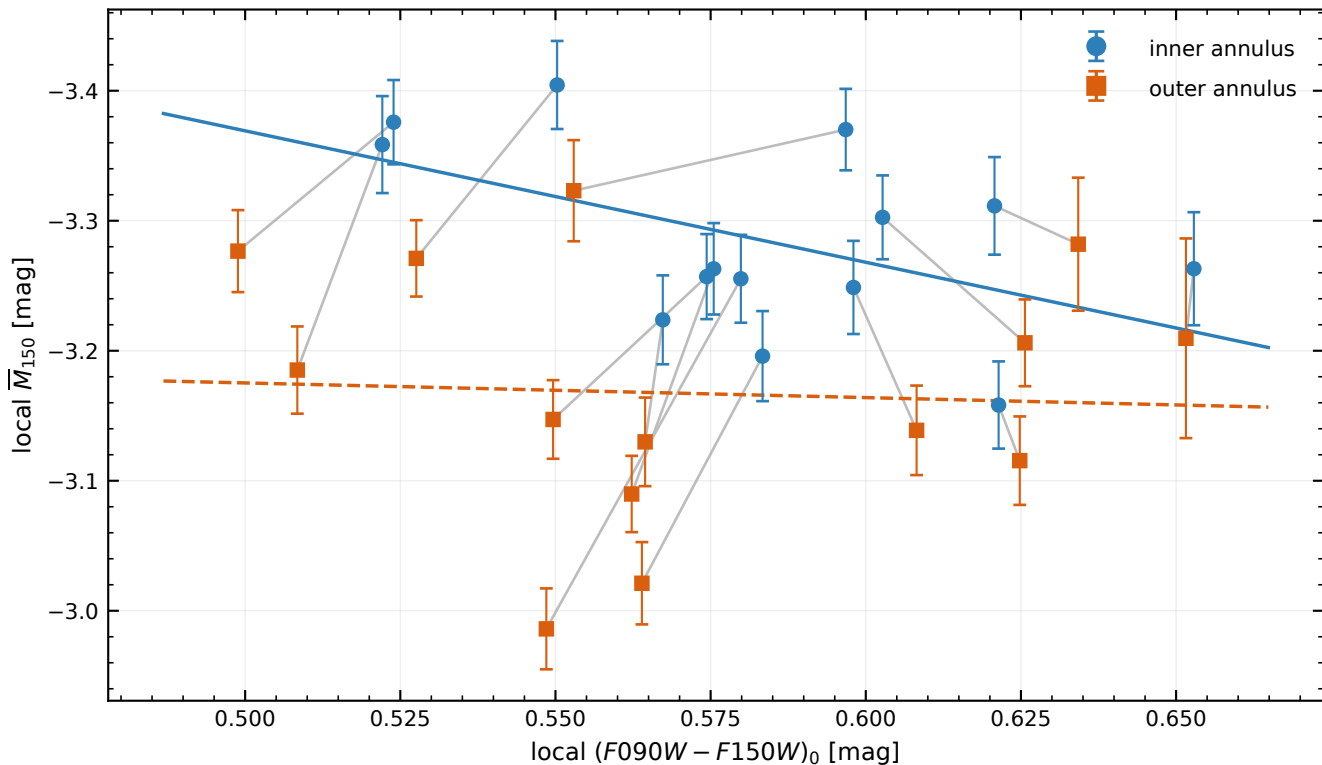
F150W annulus-matched colour and SBF
