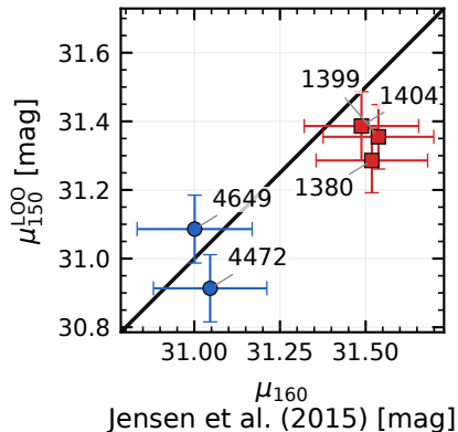
SBF distance comparison
