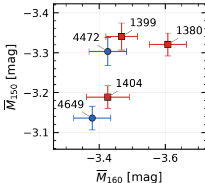
Absolute SBF with the same TRGB anchor
