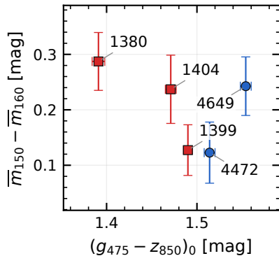
Distance-free fluctuation colour
