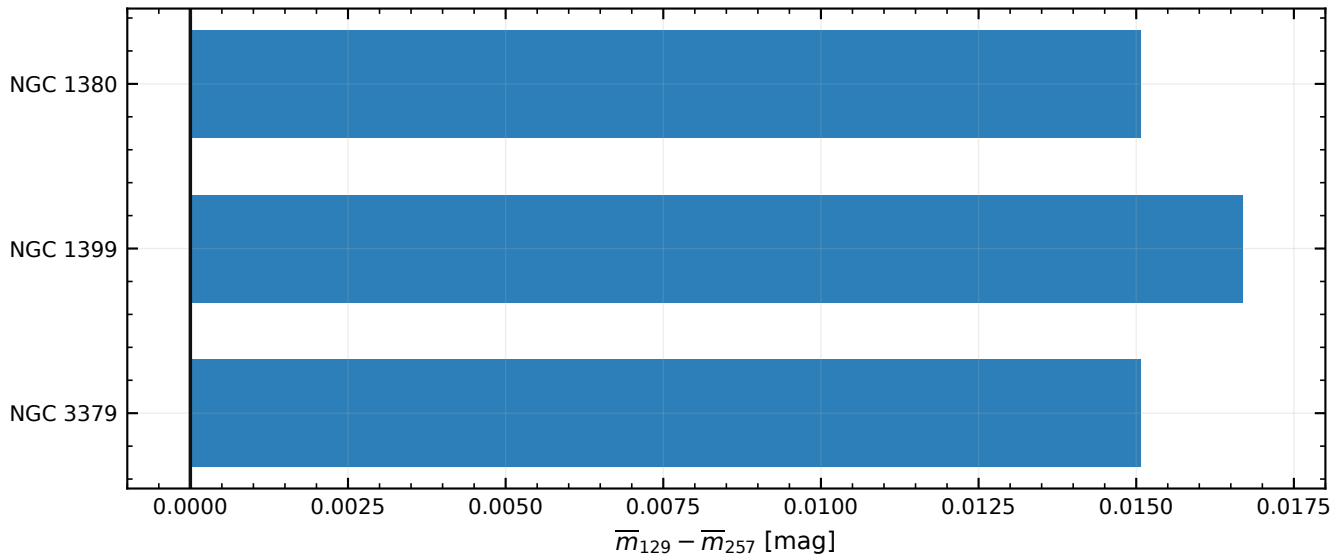
F150W PSF stamp-size sensitivity
