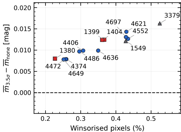
F090W: outer annulus
