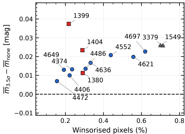
F090W: inner annulus
