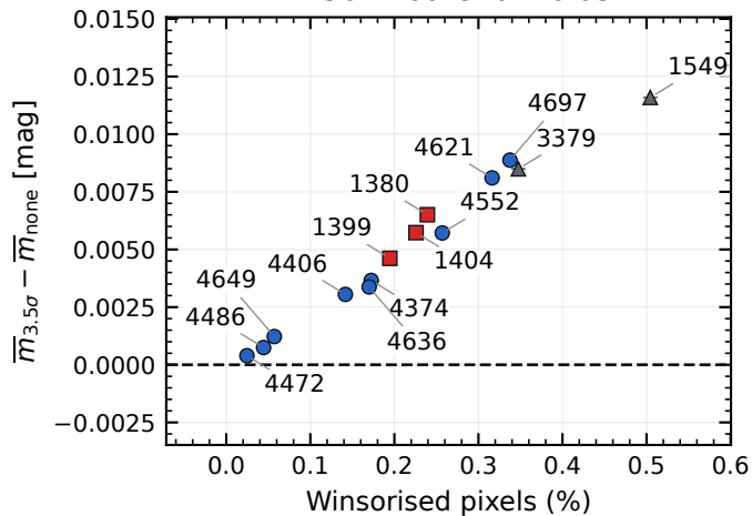
F090W: outer annulus
