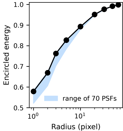
F150W: encircled energy
