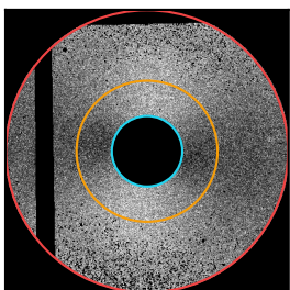
NGC 4649
