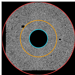
NGC 4374
