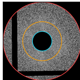
NGC 4472
