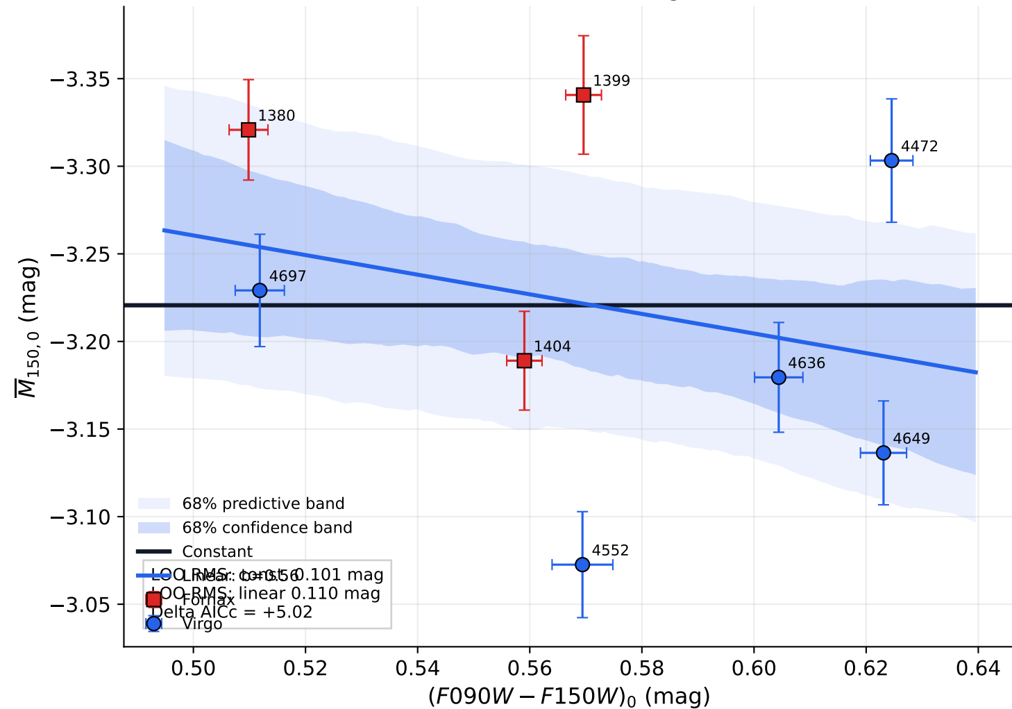
Our F150W: the same 8 galaxies
