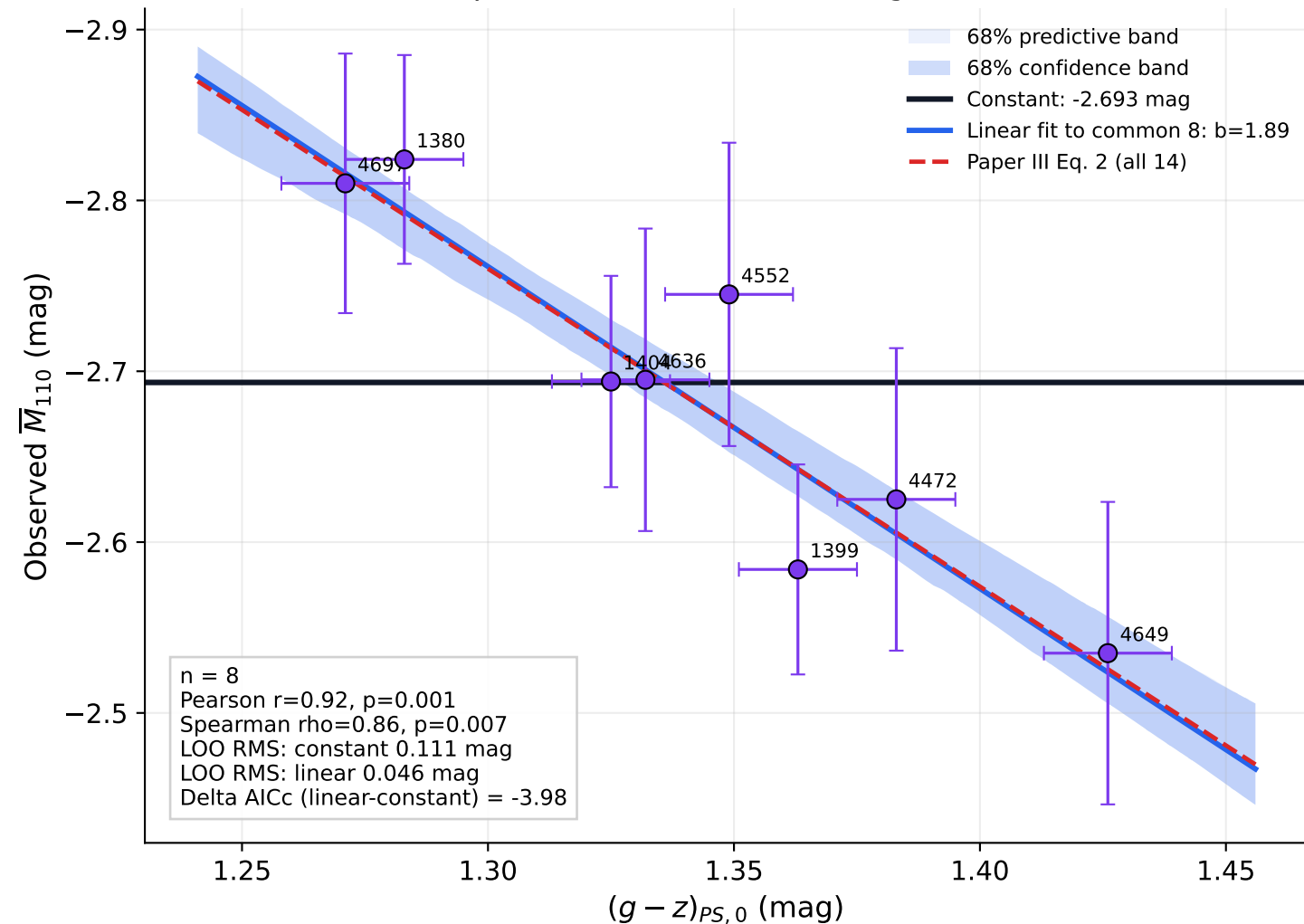
Paper III F110W: the same 8 galaxies
