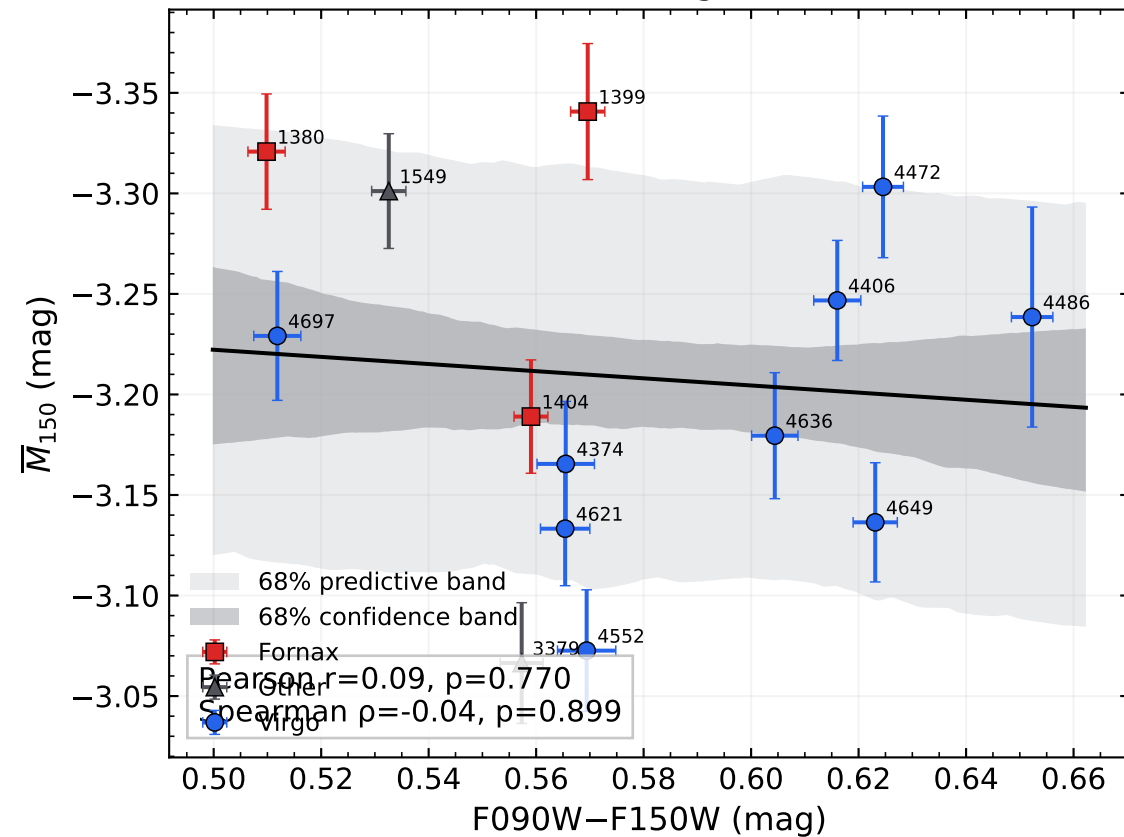
GO-3055: 14 galaxies
