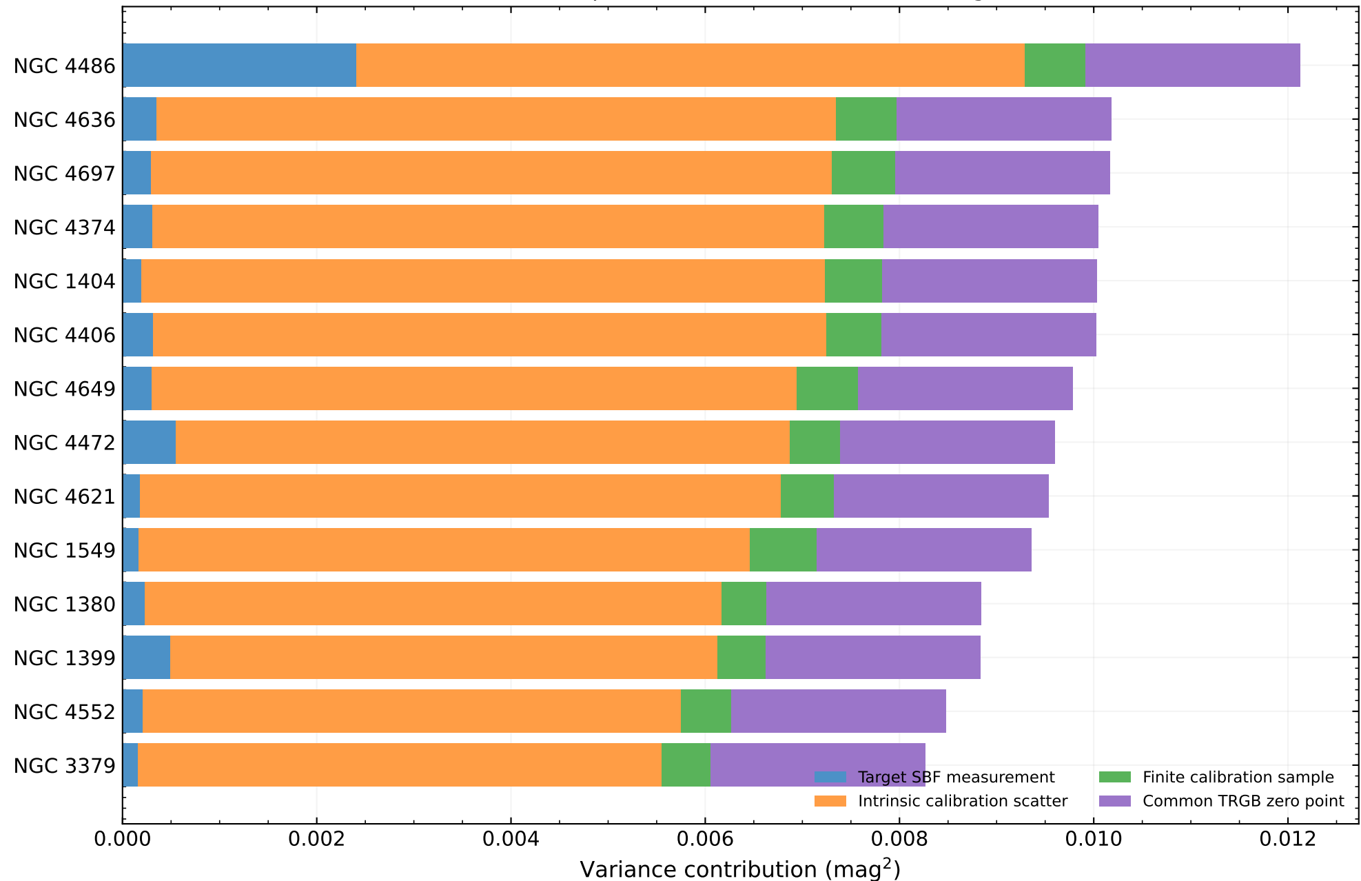
Color-independent SBF distance error budget
