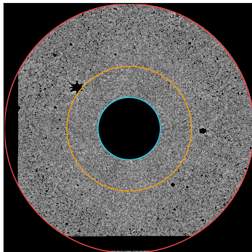
NGC 4374
