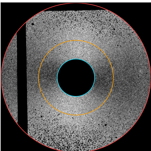
NGC 4649
