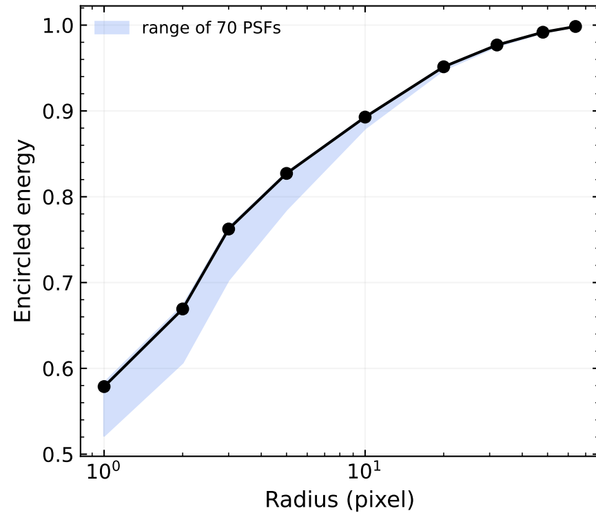
STPSF curve of growth
