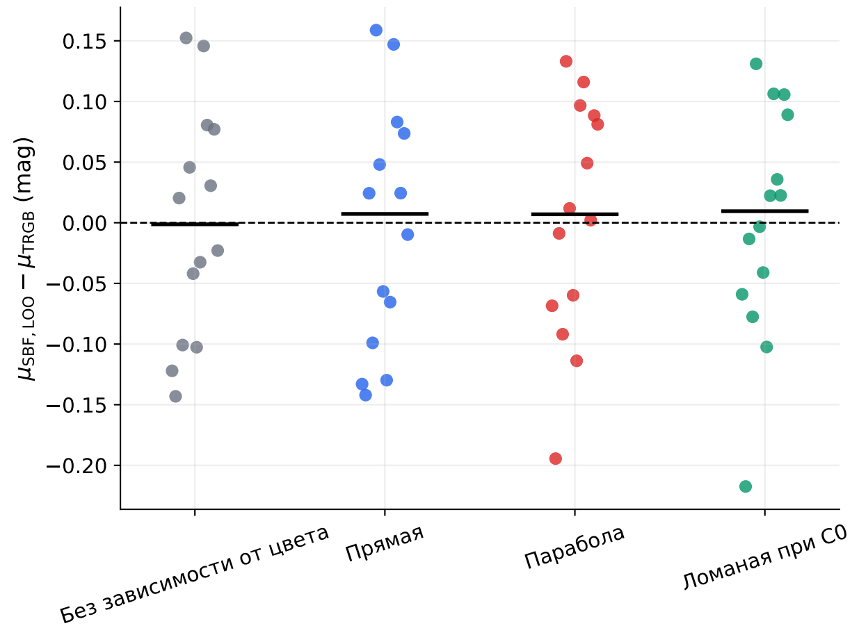
Leave-one-out residuals
