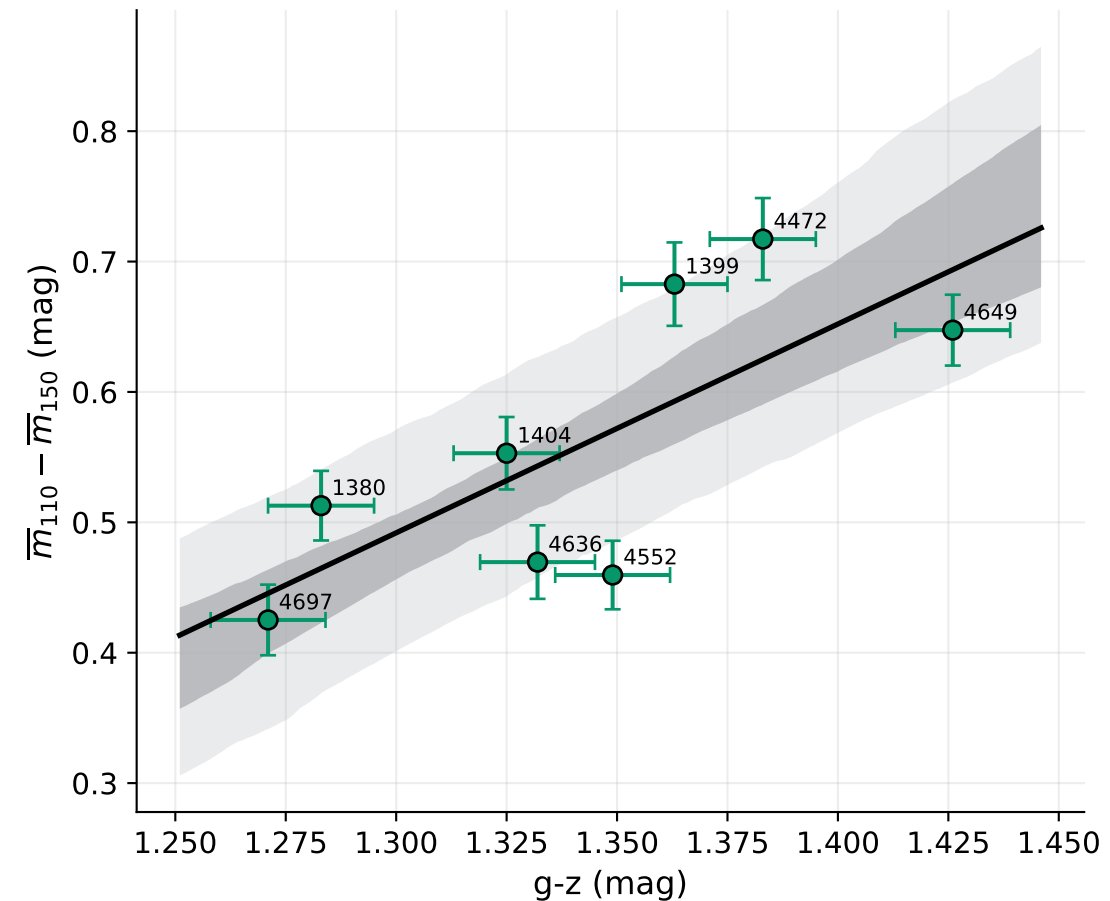
Distance-free fluctuation color
