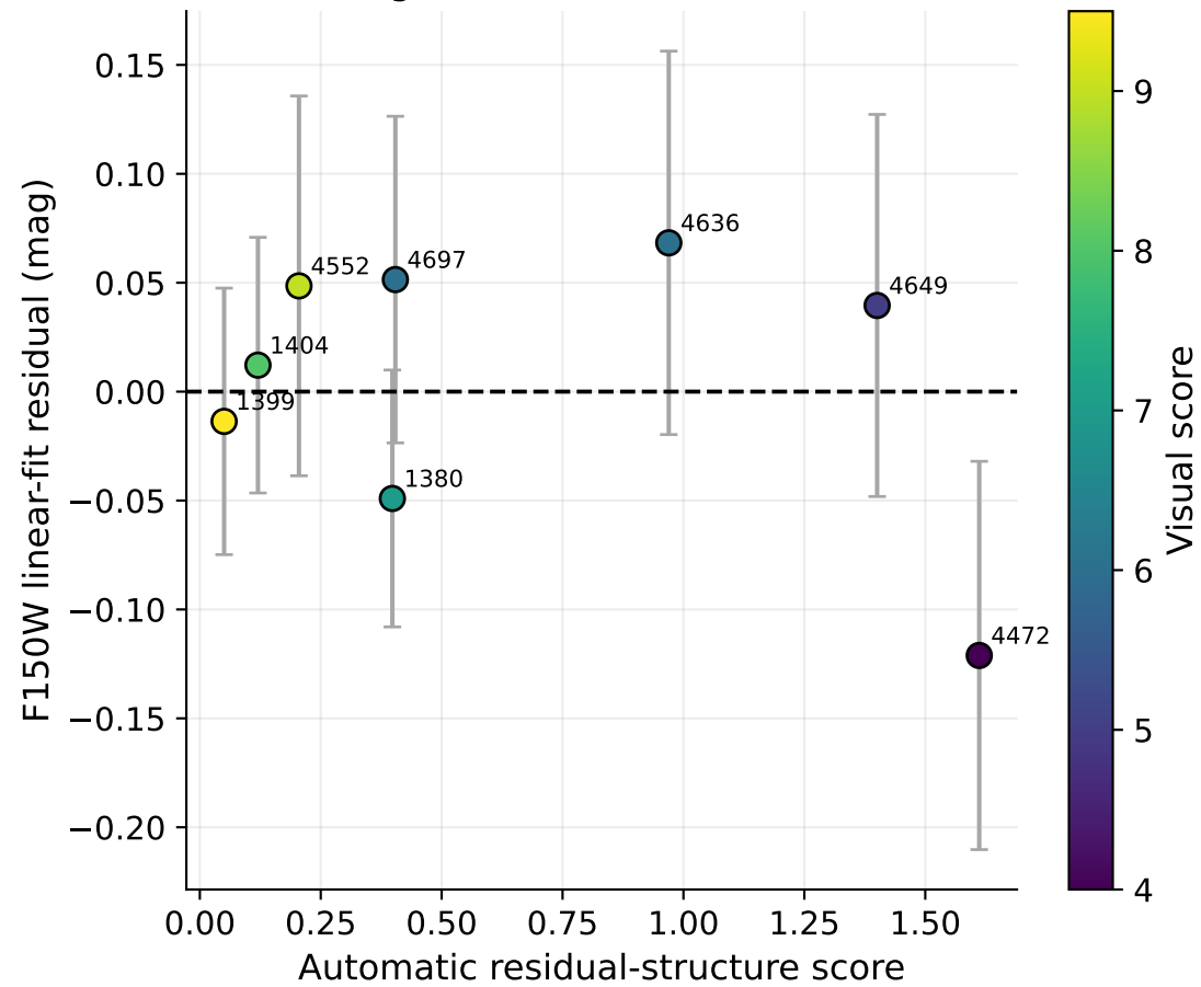
Does image structure create the scatter?
