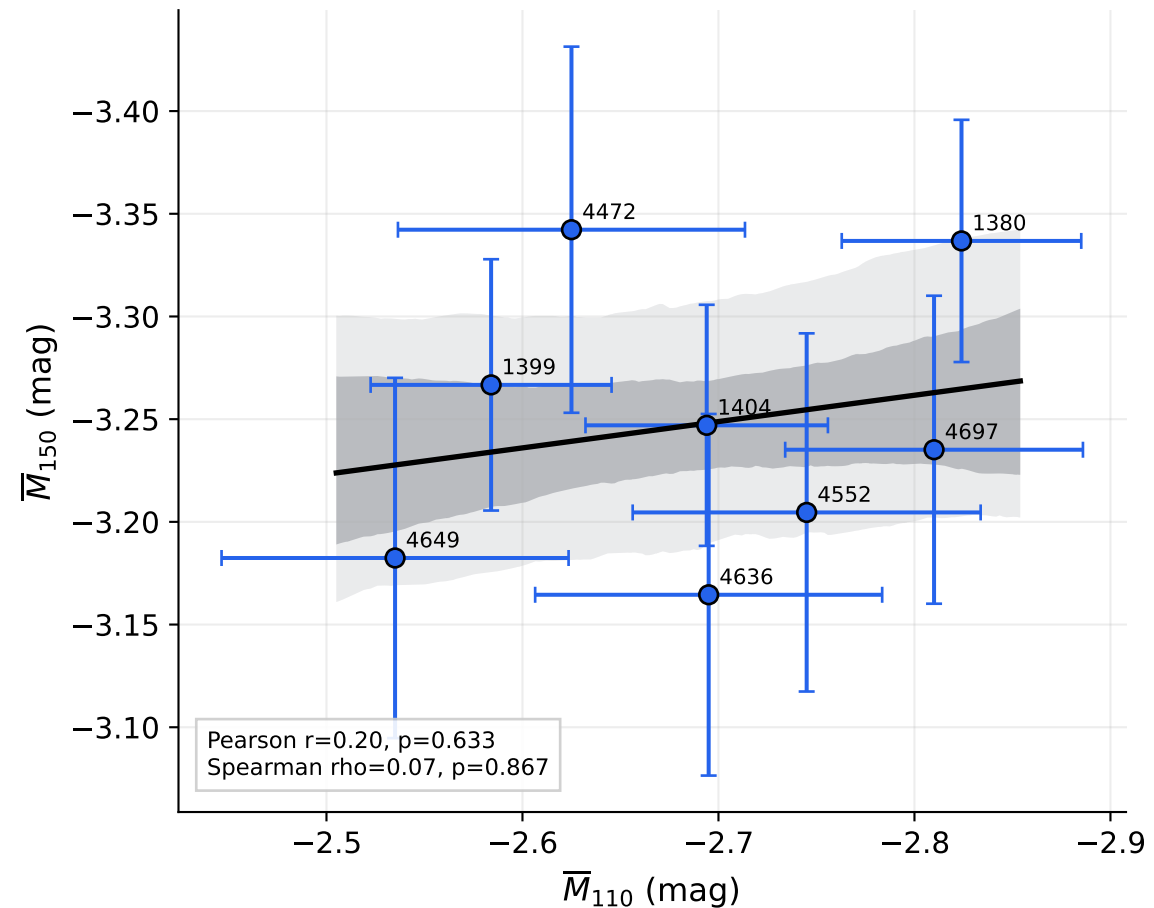
F150W versus F110W (common cluster anchor)
