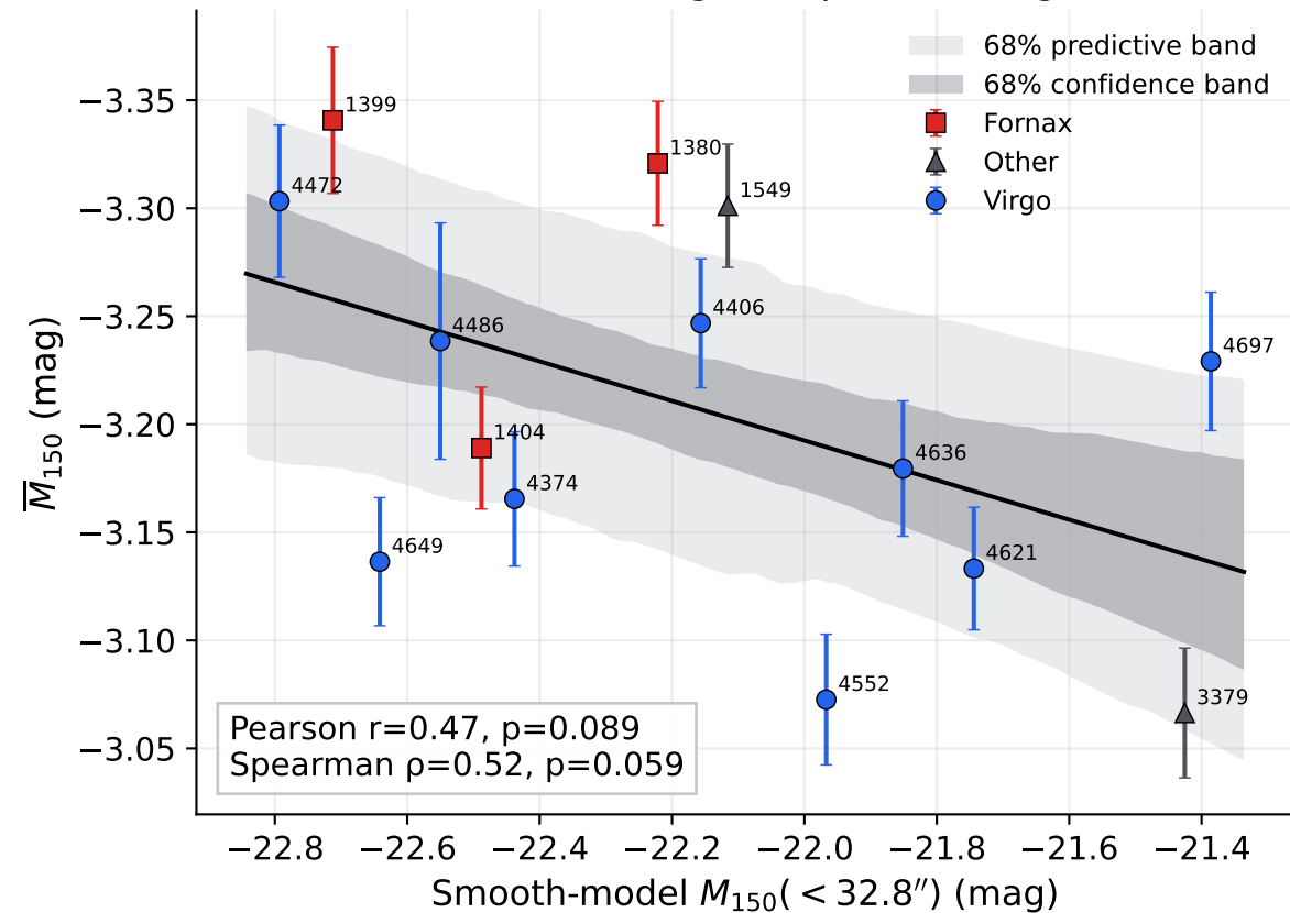
SBF versus fixed-angular-aperture magnitude
