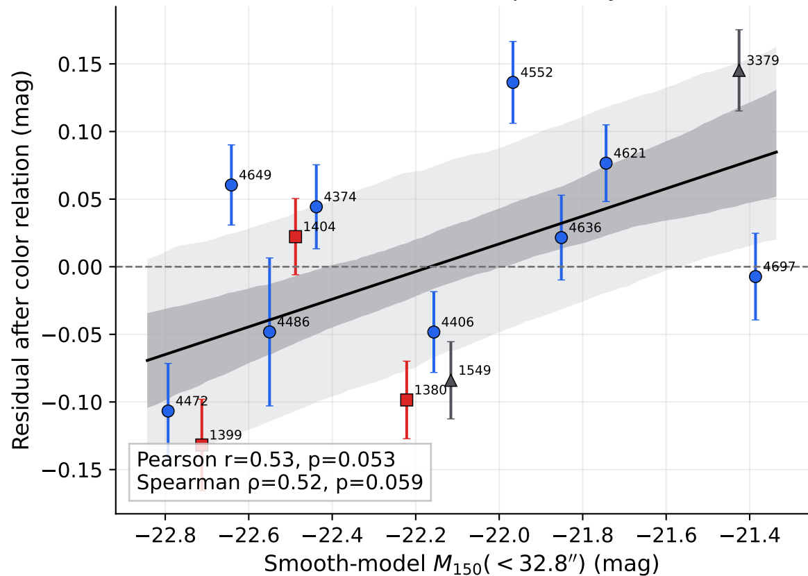
Residual trend (exploratory)
