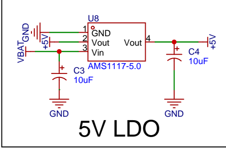
Strat Circuit
