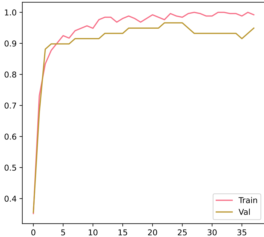
Accuracy
