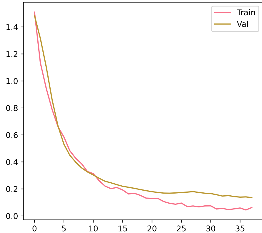
Loss
