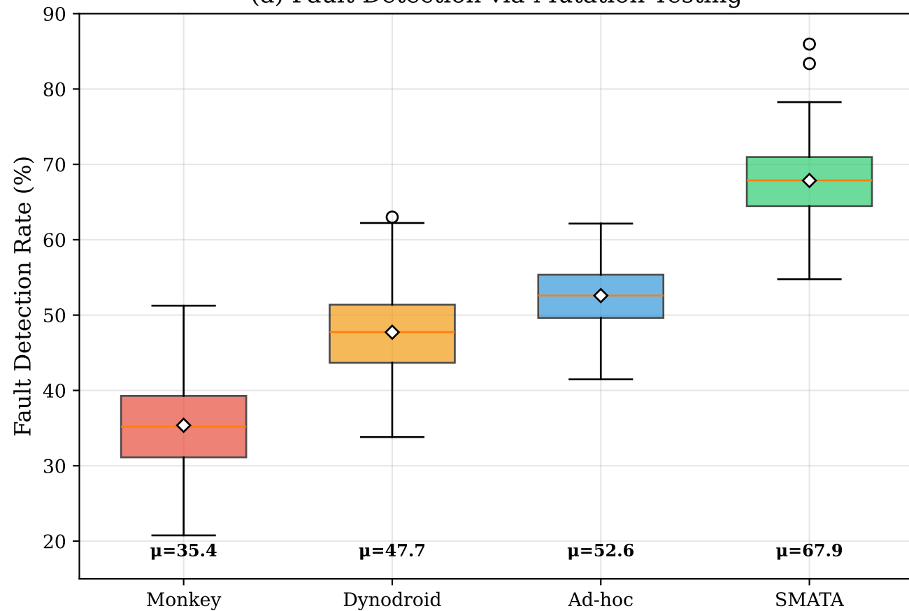
(a) Fault Detection via Mutation Testing
