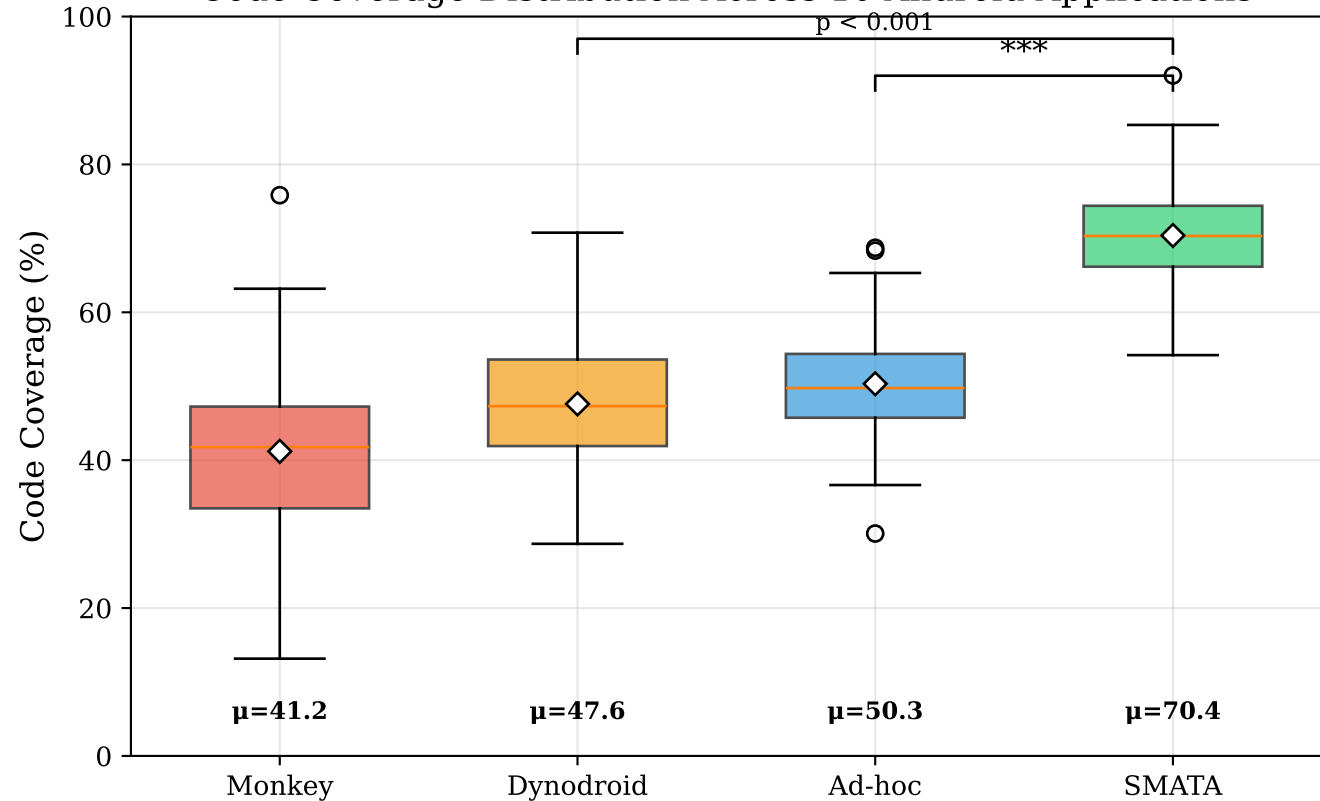
Code Coverage Distribution Across 10 Android Applications
