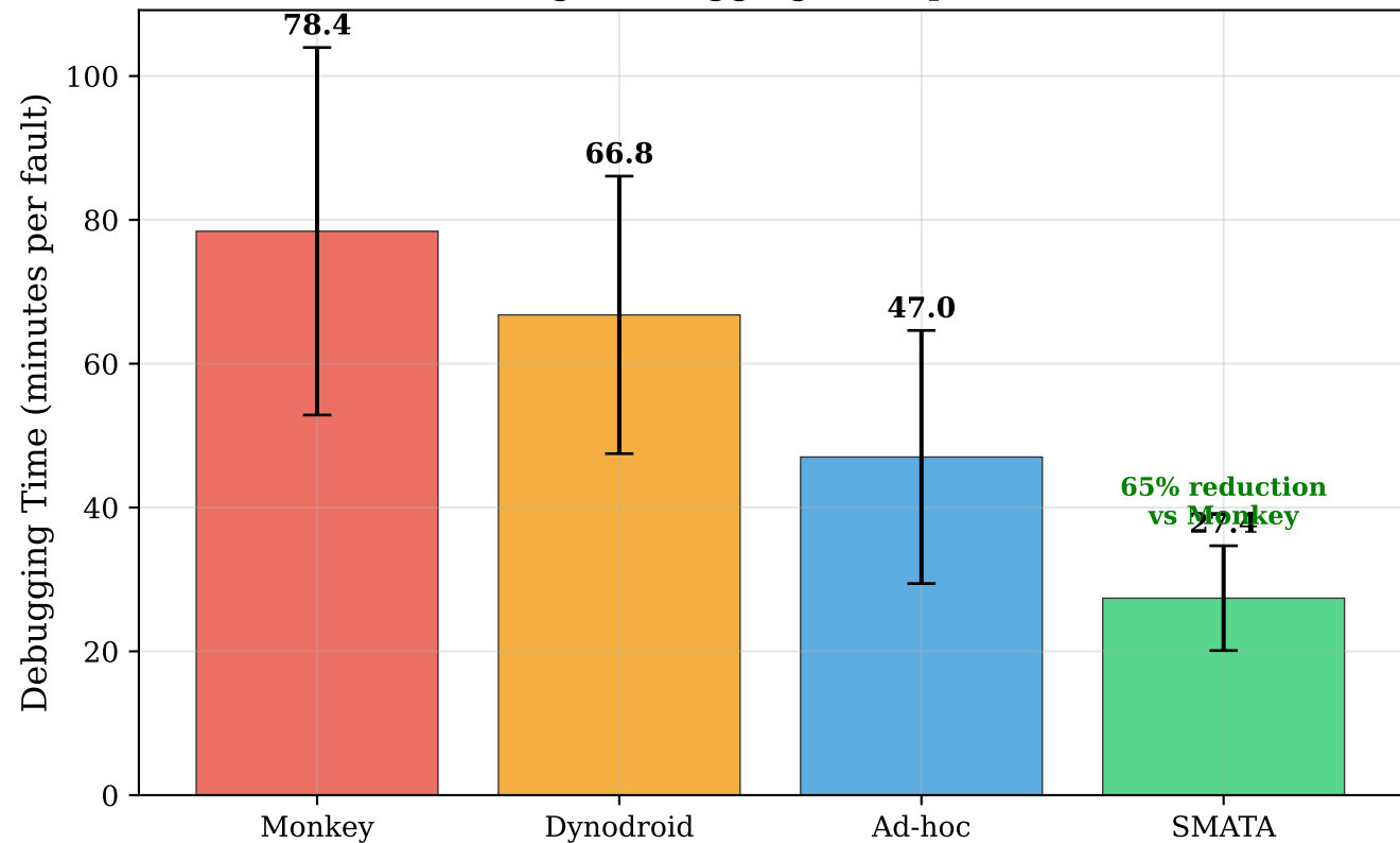
Average Debugging Time per Fault
