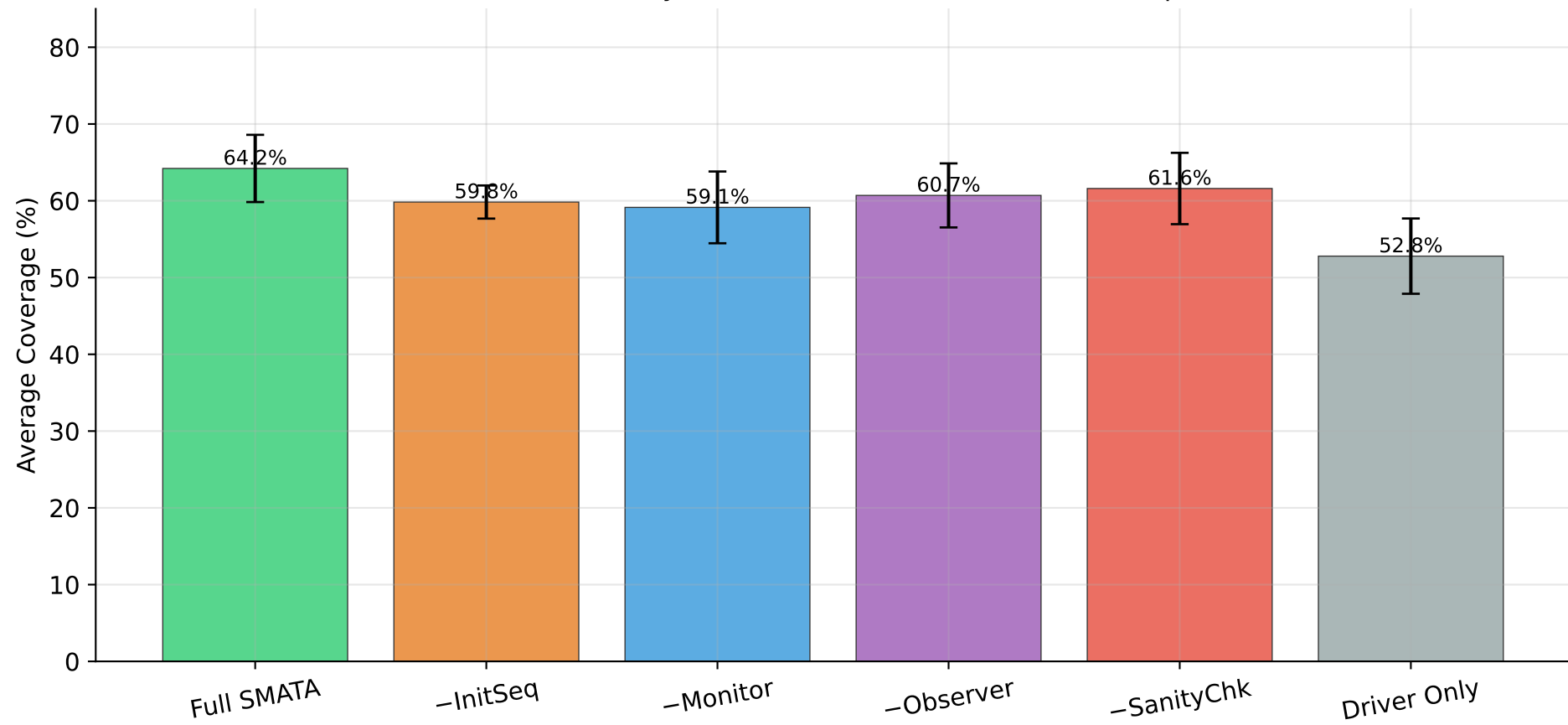
RQ4: Ablation Study — Contribution of Each SMATA Component
