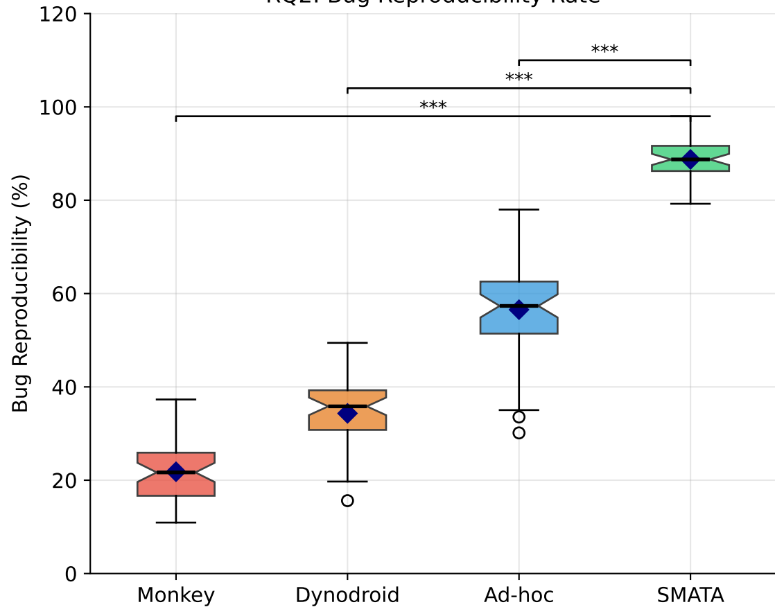
RQ2: Bug Reproducibility Rate
