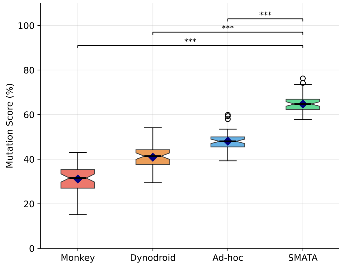
RQ2: Fault Detection Rate
