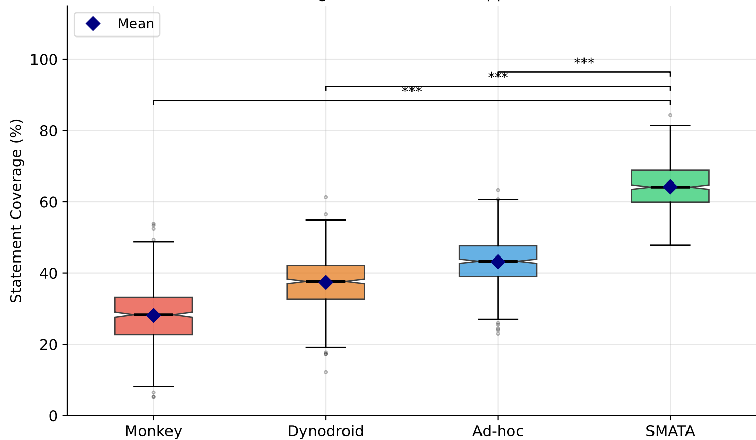
RQ1: Code Coverage Distribution (50 Apps × 10 Runs Each)
