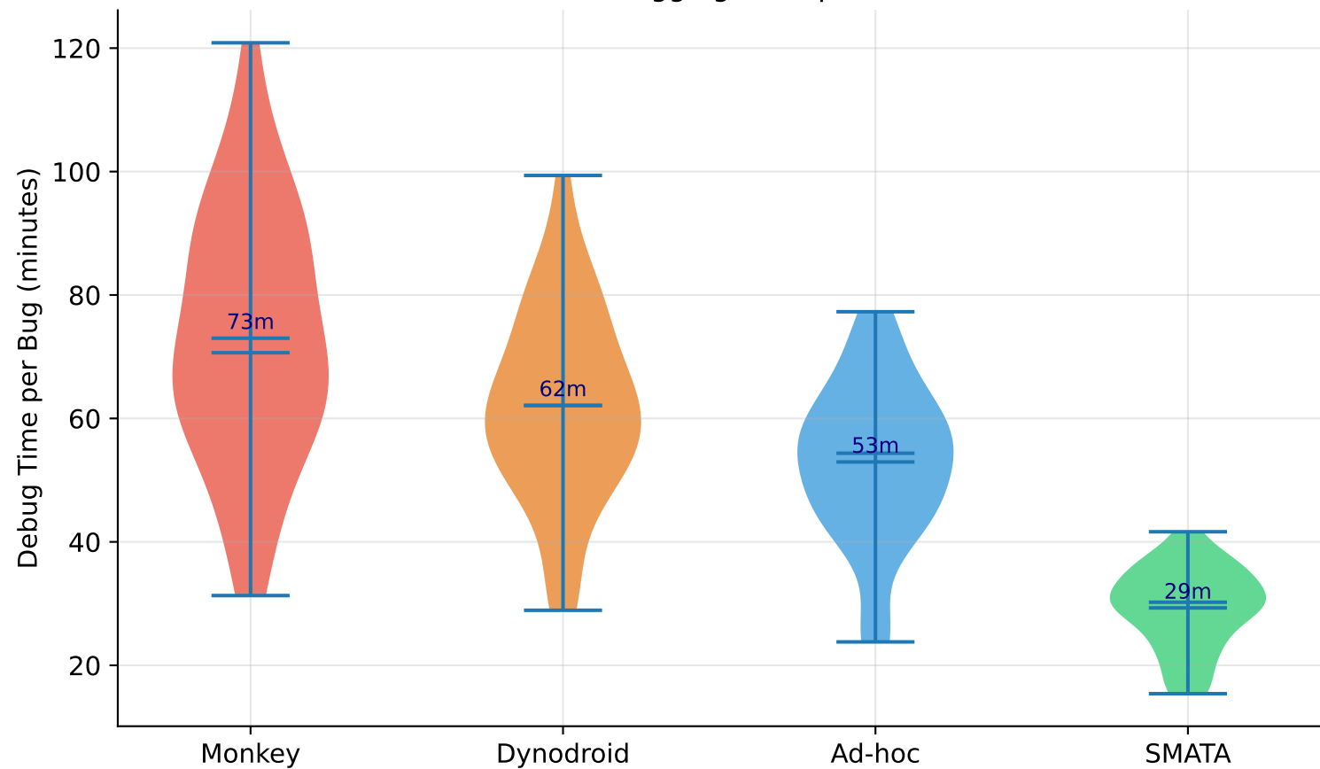
RQ2: Debugging Time per Fault
