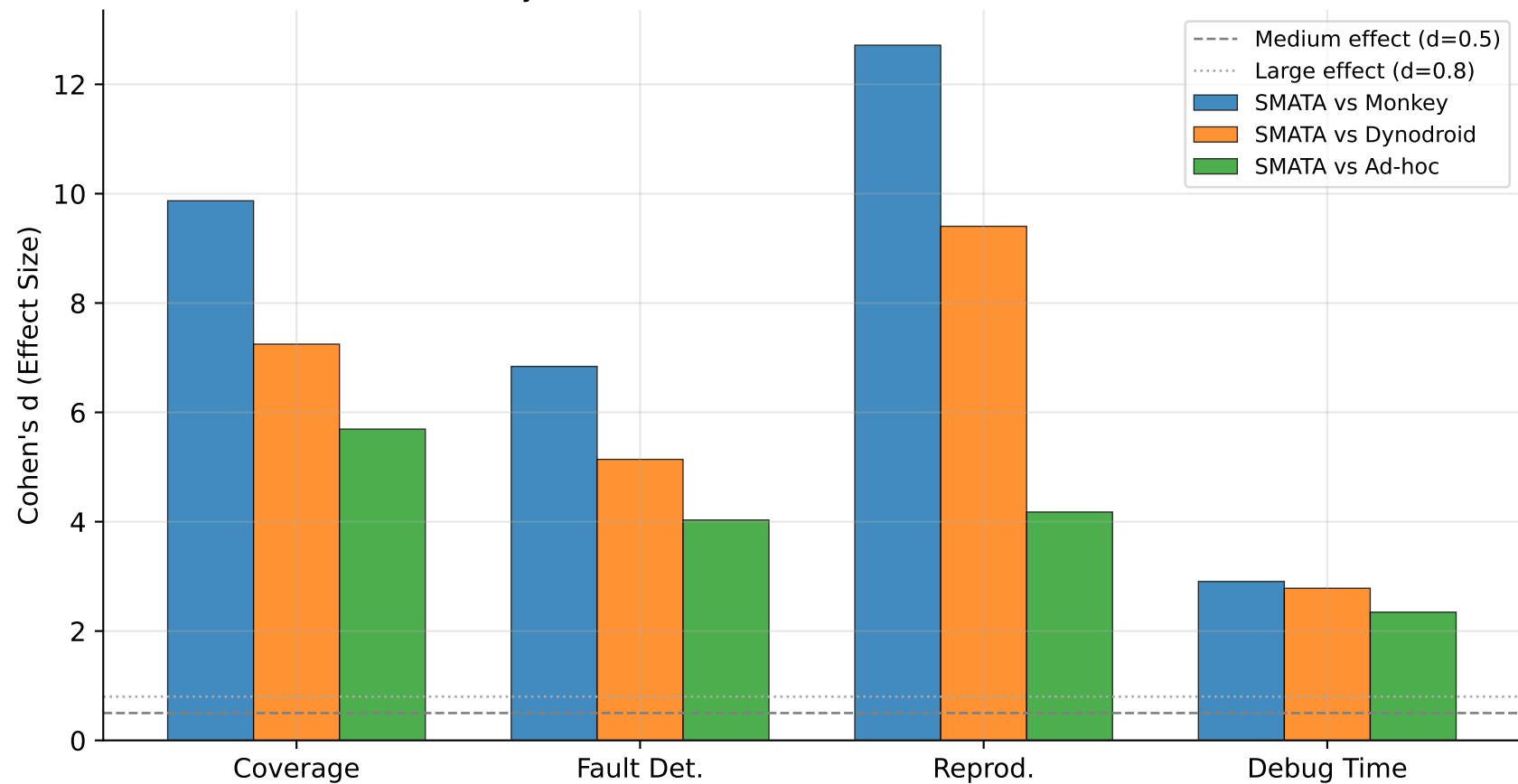
Summary of Effect Sizes Across All Metrics and Baselines
