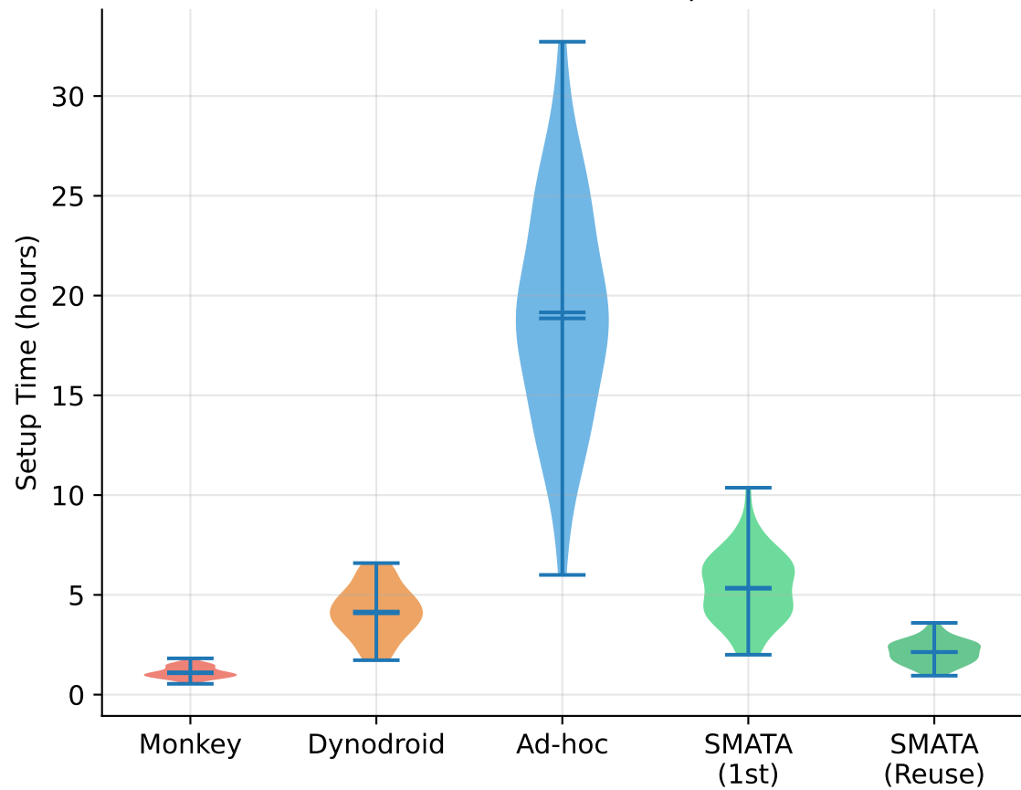
RQ3: Distribution of Setup Times
