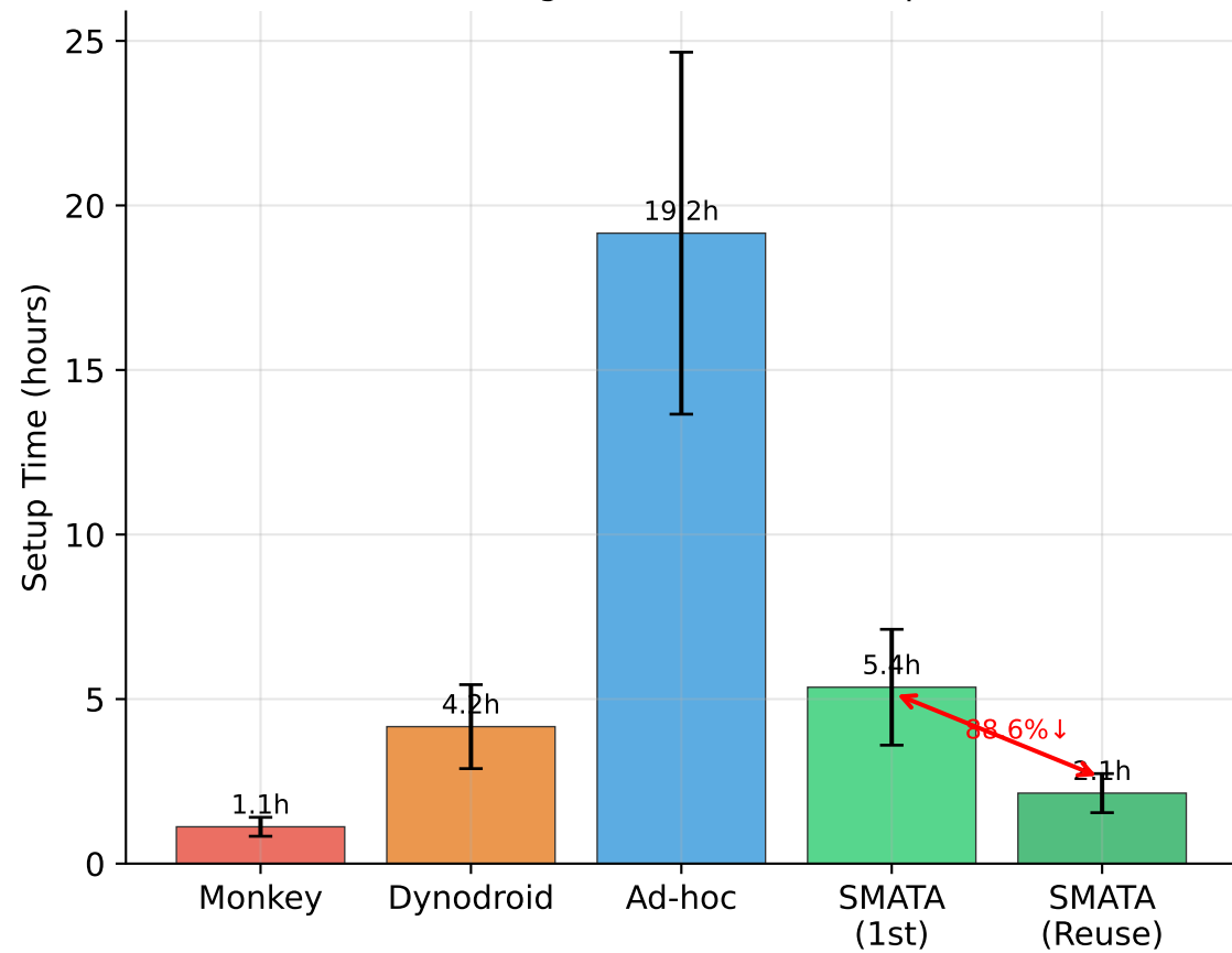
RQ3: Testing Infrastructure Setup Time
