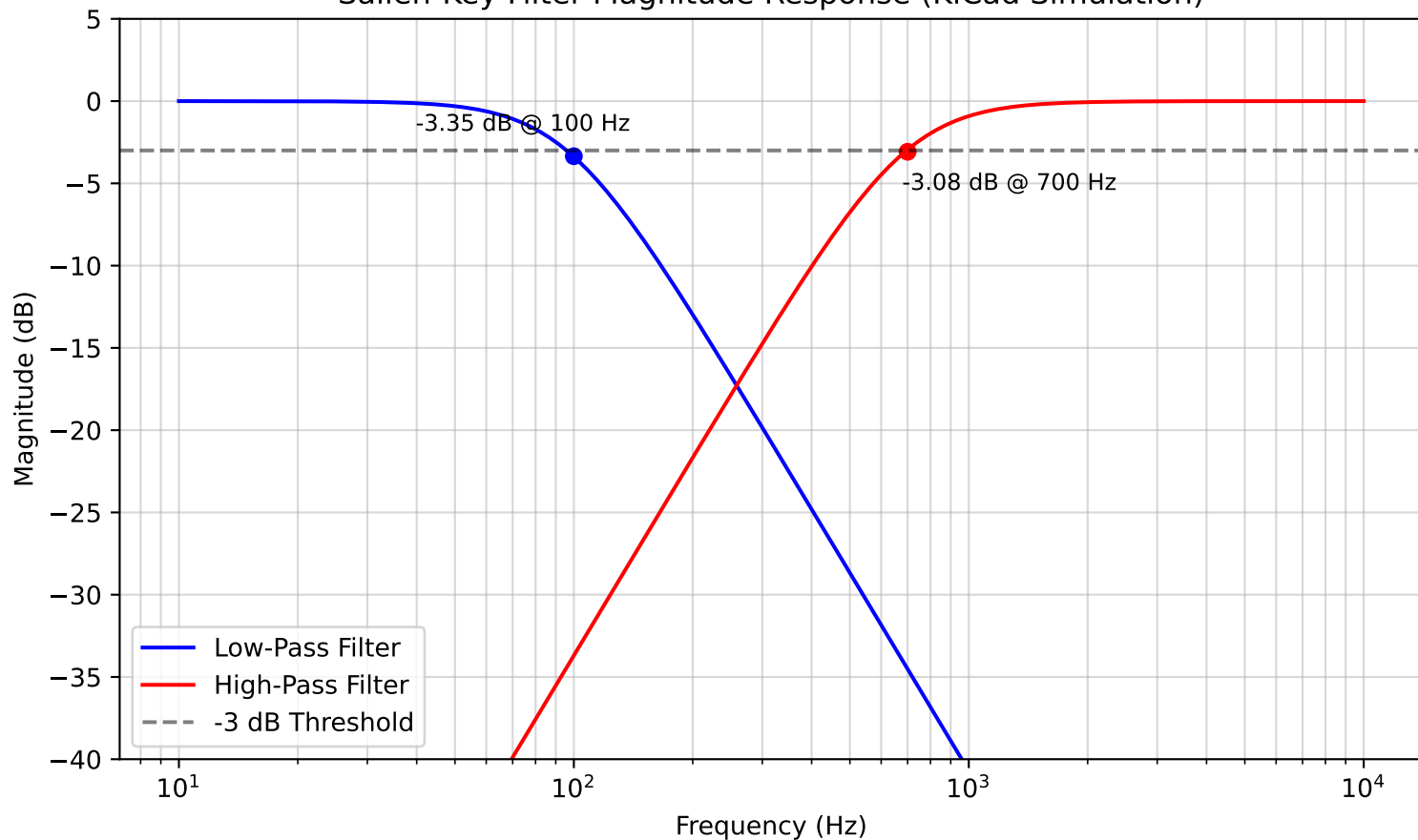
Sallen-Key Filter Magnitude Response (KiCad Simulation)
