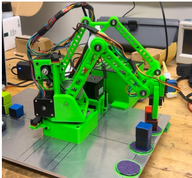
Figure 2.9: Robot during operation; cubes sorted and stacked by color
