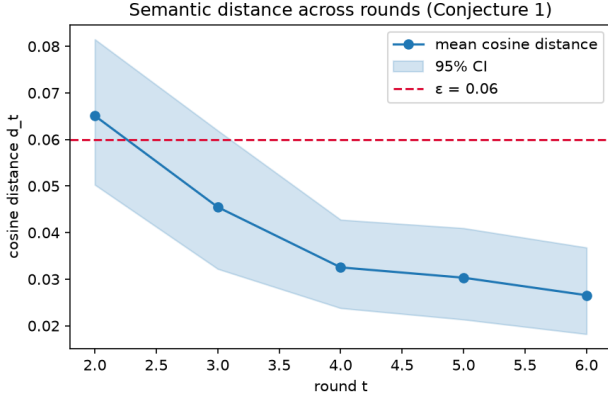
Fig. 5. Mean semantic distance d_t versus round, with a 95% confidence band (test split, N = 60 ). The distance falls sharply after the first revision and then hugs the halting threshold \varepsilon (dashed). The decreasing trend is statistically significant (Conjecture 1), while the heavy tail justifies the patience window.
