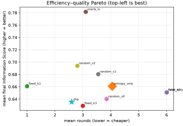
Fig. 3. Efficiency-quality Pareto (development split). Quality is only weakly tied to rounds; the oracle sits far above every practical policy, and full shp is dominated. Top-left is best.
