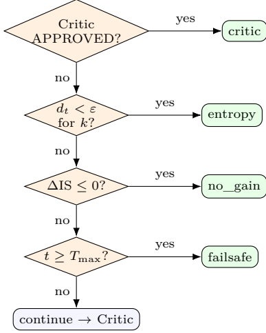
Fig. 2. Priority-ordered halt cascade. Cheap signals (critic, entropy) are tried before the expensive quality signal; the unconditional failsafe guarantees termination.
