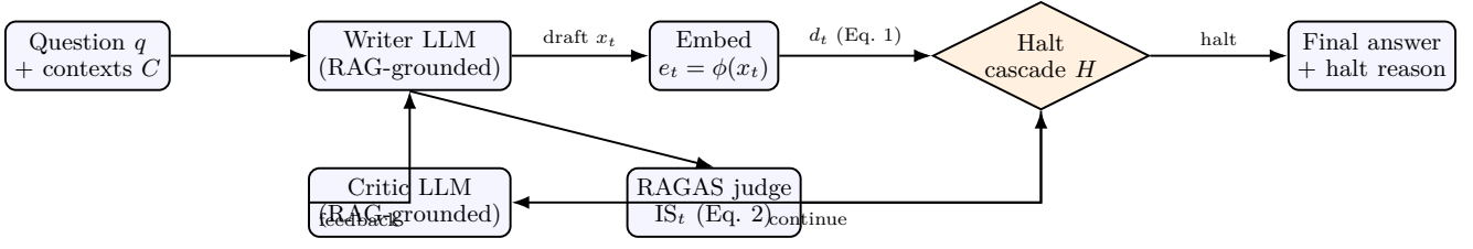
Fig. 1. SHP architecture. The Writer and Critic both condition on the retrieved contexts (a genuine RAG setting). Embeddings are computed by a local model and are therefore free; only the RAGAS judge consumes API tokens. The halt cascade H reads the cheap geometric signal d_t , the critic verdict, and—only when required—the quality signal IS_t .
