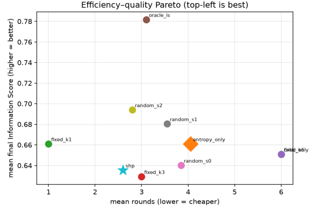
Fig. 3. Efficiency–quality Pareto (development split). Quality is only weakly tied to rounds; the oracle sits far above every practical policy, and full shp is dominated. Top-left is best.
