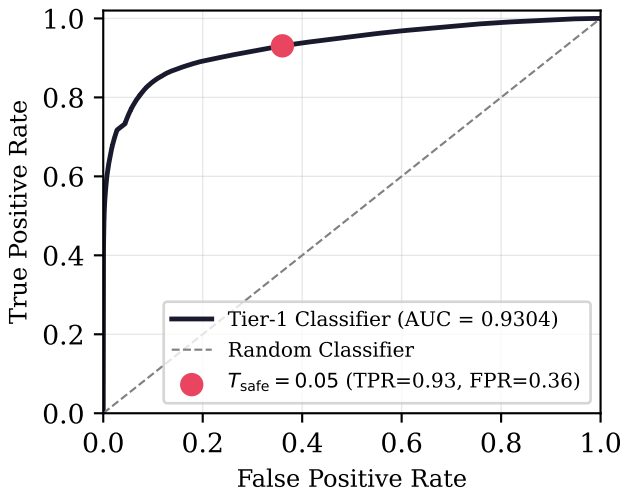
ROC Curve --- Tier-1 Calibrated XGBoost
