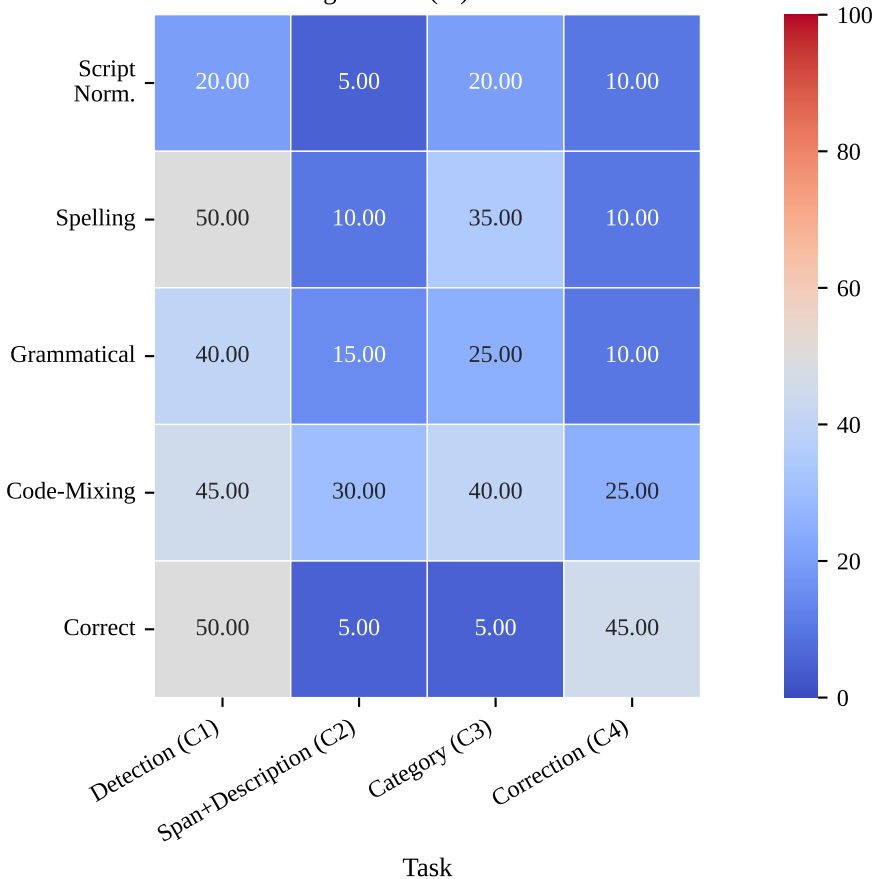
Exact Agreement (%) — All Raters
