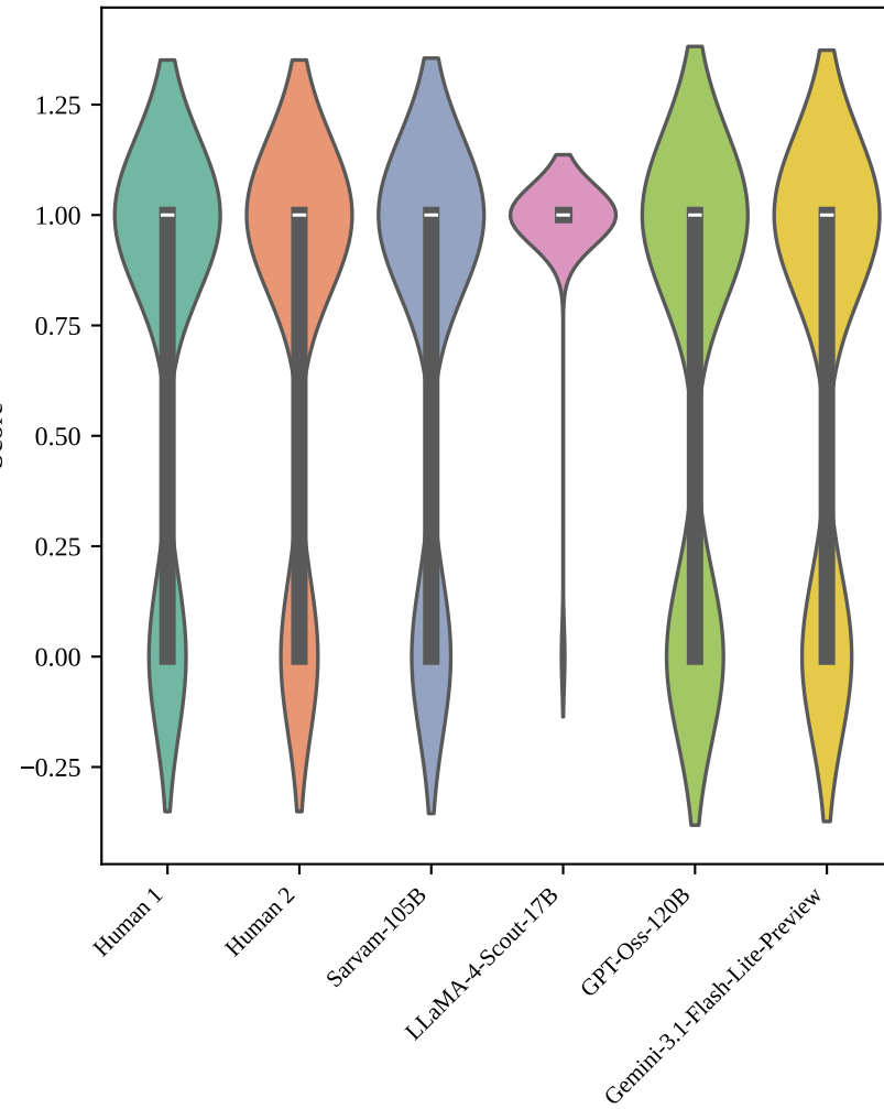
Detection (C1)
