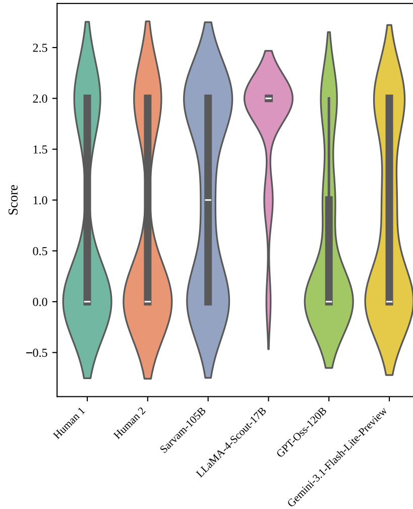
Span+Description (C2)
