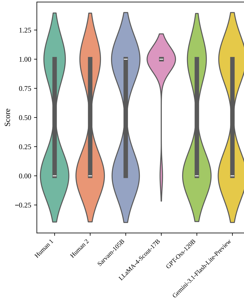
Category (C3)
