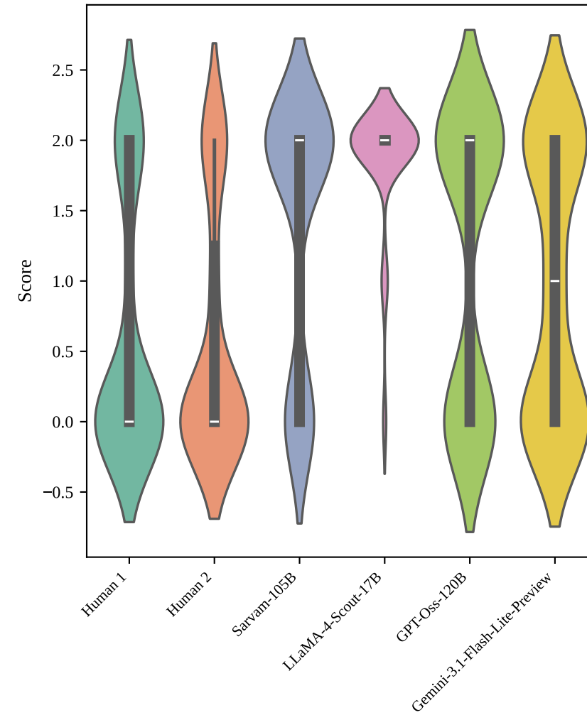
Correction (C4)
