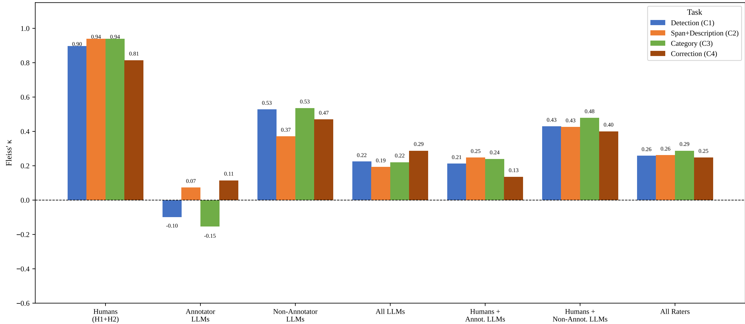
Fleiss' \kappa by Rater Group and Task
