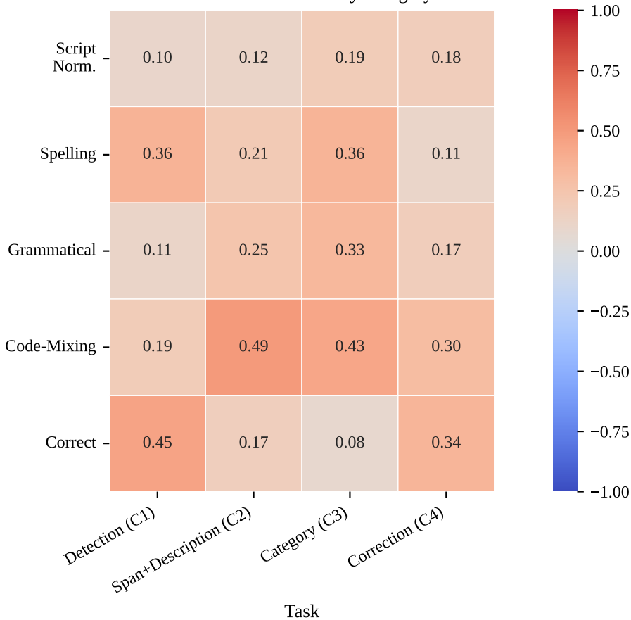
Fleiss' \kappa — All Raters by Category
