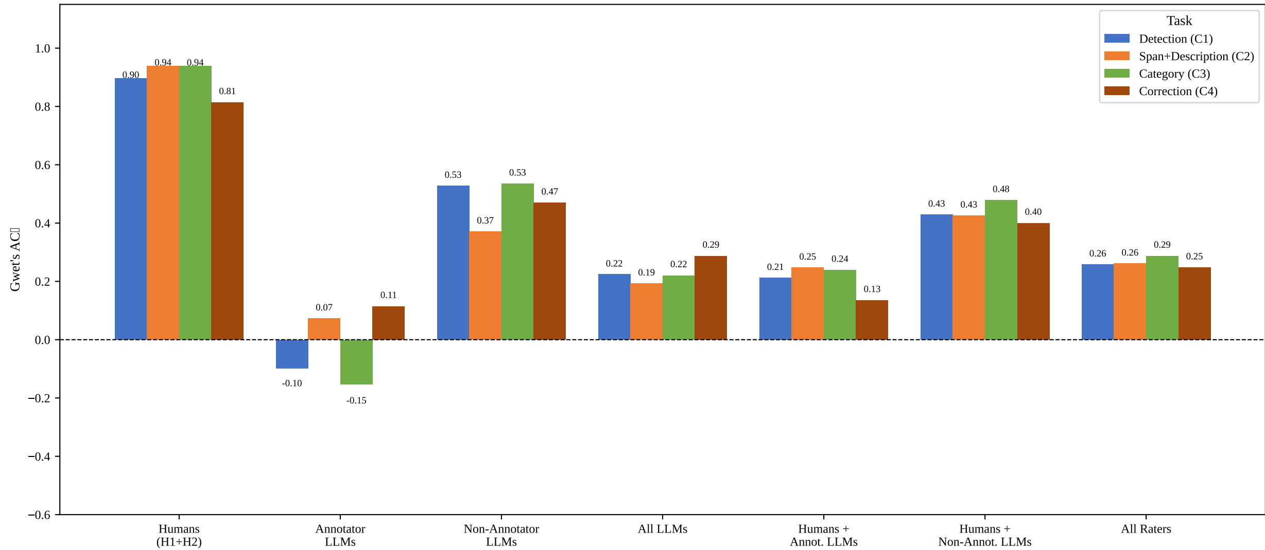
Gwet's AC \kappa by Rater Group and Task
