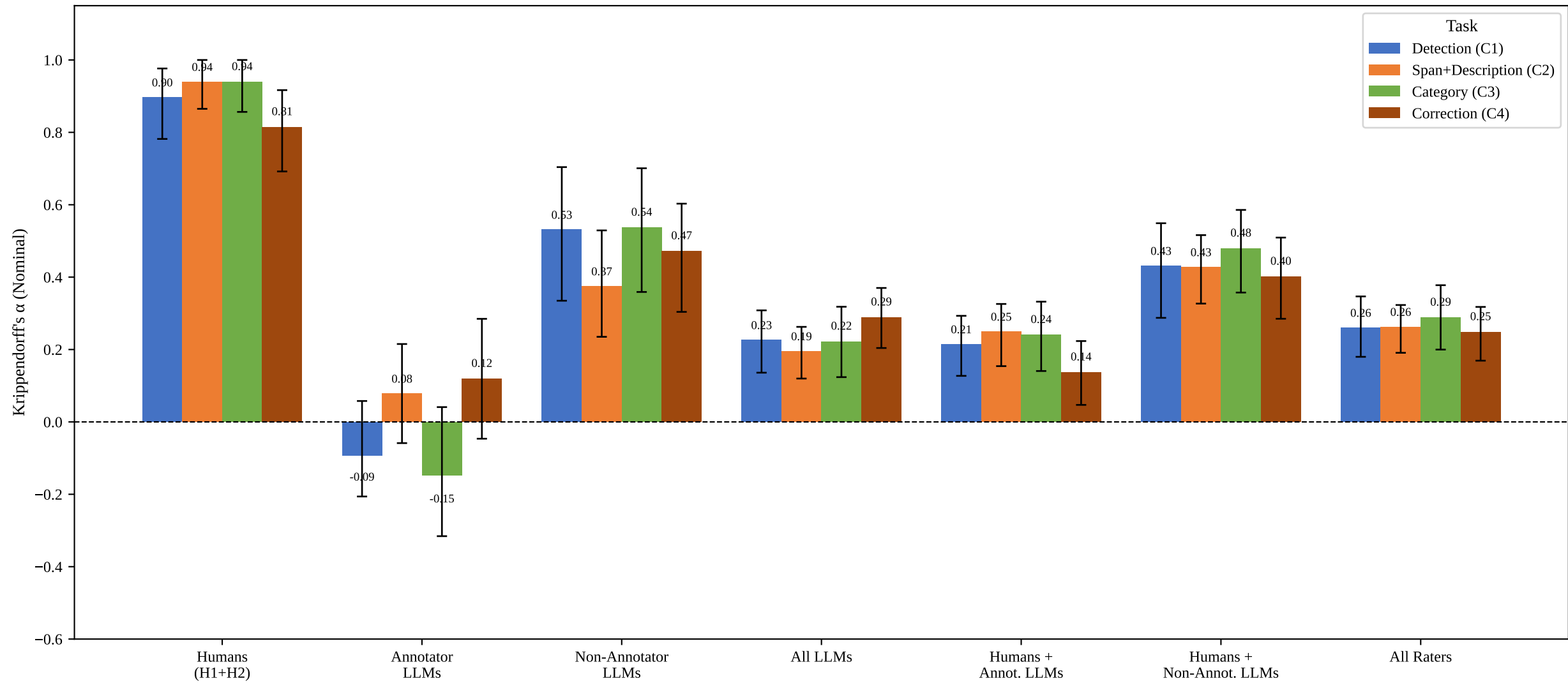
Krippendorff's \alpha (Nominal) with 95% CI
